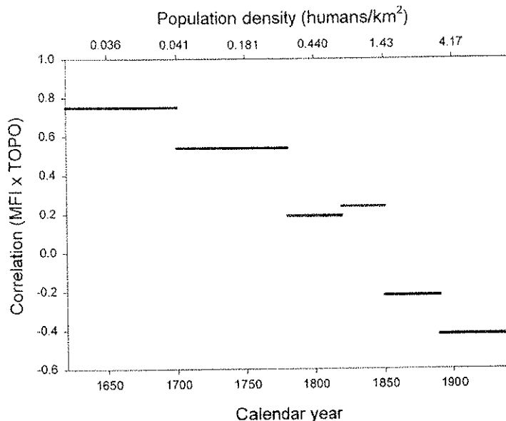
Figure 4.—This graph illustrates how human population density can mitigate the effects of topographic roughness on the frequency of fire. The y axis is the correlation coefficient between fire frequency (MFI) and the Index of Topographic Roughness. The upper x axis shows the mean population density of the period of correlation. The bars indicate the level, sign, and period of the correlation calculation. Correlations for the two earliest and the latest periods are significant ( p < 0.05 ).
