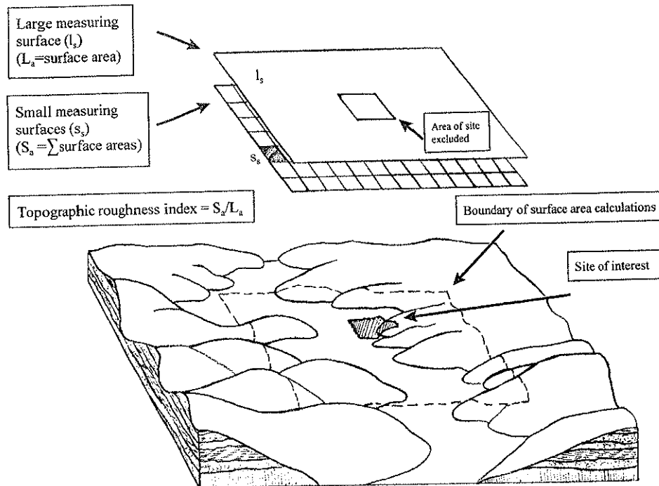
Figure 1.—Topographic roughness is an important variable which interacts with human population density to control the frequency of fire. Topographic roughness can be estimated with an Index of Topographic Roughness. The illustrated example of an Index of Topographic Roughness is calculated by measuring the circumscribed region of the earth of a given dimension and shape with a large measuring surface ( L_s ) and many small measuring surfaces ( s_s ). The sum of the areas ( S_s ) of the small measuring surfaces is then divided by the area ( L_s ) of the large measuring surface to obtain the Index of Topographic Roughness.
