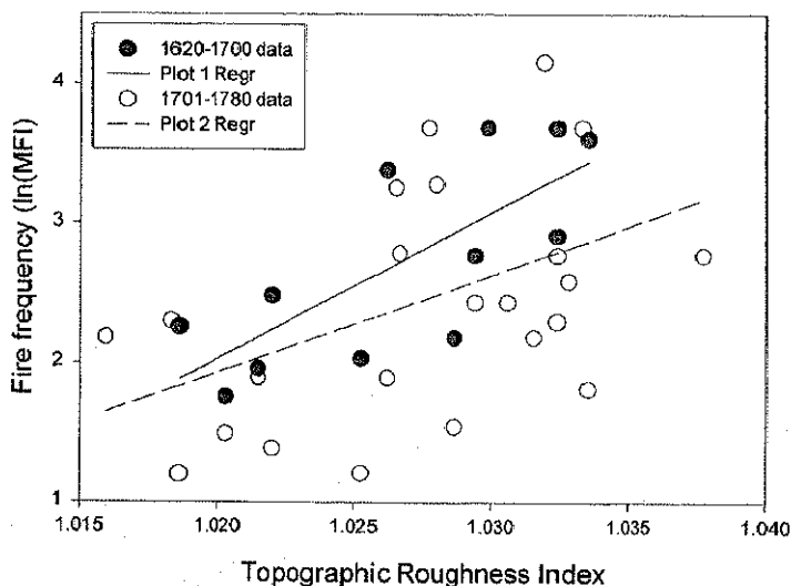
Figure 3.—These two scatter plots and regression lines illustrate the mitigation of fire frequency (MFI) by topographic roughness during two periods of low human population density. Topographic roughness is hypothesized to have reduced the frequency of fire by inhibiting the ignition and spread of anthropogenic fires.
