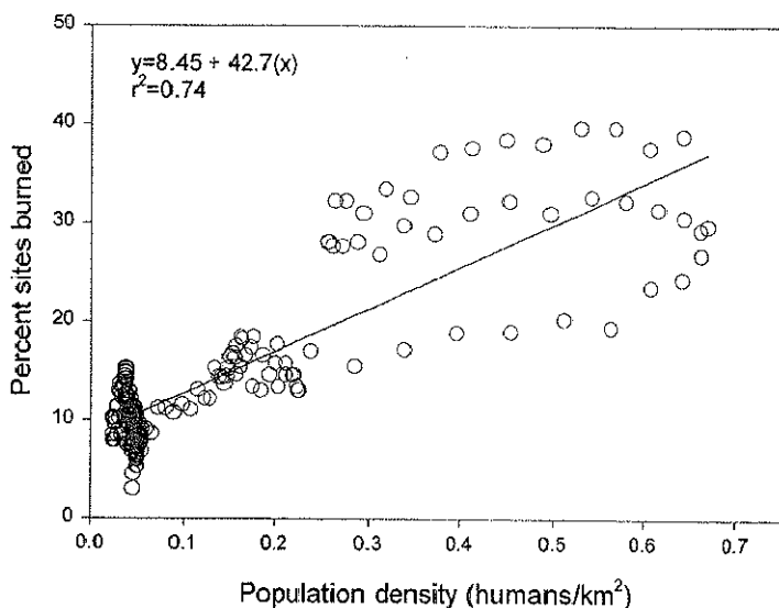
Figure 2.—Human population density is the major factor in the frequency of wildland fire ignitions in many regions. This scatter plot and regression illustrate the change in the percentage of study sites burned each year with human population density. The data is for the period 1620 to 1850 and is from the Current River watershed in Missouri. The percentage of sites burned (y axis) is from annual data that has been smoothed with an 11 year moving average (Guyette and Cutter 1997).
