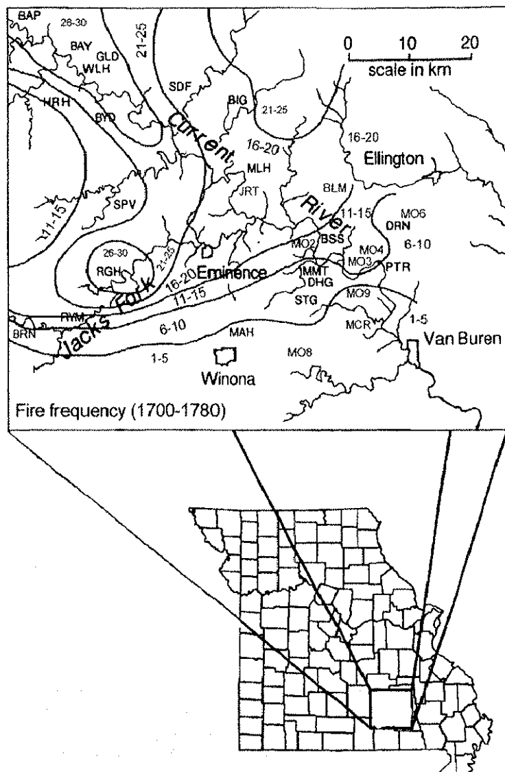
Figure 5.—This map illustrates the diversity of mean fire intervals present at the landscape level during a period (1700 to 1780) of low to moderate population density, which best reflects the fire regime many centuries before European settlement. Fire frequency gradients are represented by the iso-pyro lines. Iso-pyro lines define a gradient of equal fire frequencies. Numbers adjacent to iso-pyro lines give the class of mean fire intervals defined by each line.
