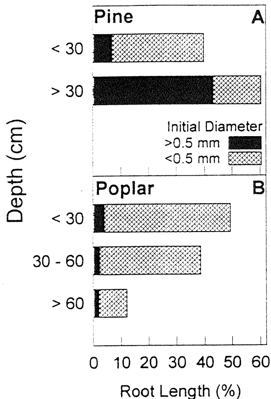
Figure 3. Percentage of total root length for pine (A) and poplar (B) in each different depth by initial root diameter category. Initial root diameters represent fine feeder roots ( <0.5 mm) and pioneer roots ( >0.5 mm). Percentages are based on root length in each depth by size category compared to total root length per minirhizotron. Values are the means of four replicate minirhizotrons. See Table 2 for statistical analysis.
