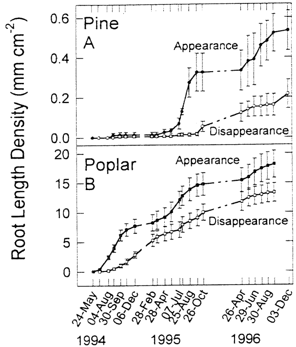
Figure 1. Cumulative root length density appearance and disappearance for pine (A) and poplar (B) over three growing seasons. Each point is the mean \pm standard error ( n=4 ).
