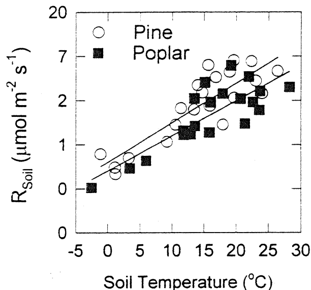
Figure 7. Soil \text{CO}_2 efflux ( R_{\text{Soil}} ) response to soil temperature ( T_{\text{Soil}} ). The linear model \ln(R_{\text{Soil}}) = B_0 + B_1 T_{\text{Soil}} was fitted for pine ( B_0 = -0.396 ; B_1 = 8.96 \times 10^{-2} ; R^2 = 0.752 ) and for poplar ( B_0 = -0.589 ; B_1 = 7.90 \times 10^{-2} ; R^2 = 0.676 ). The regression lines tested parallel and the pine model was significantly greater than the poplar model ( P -value = 0.011). Each point is the mean of four measurement locations.
