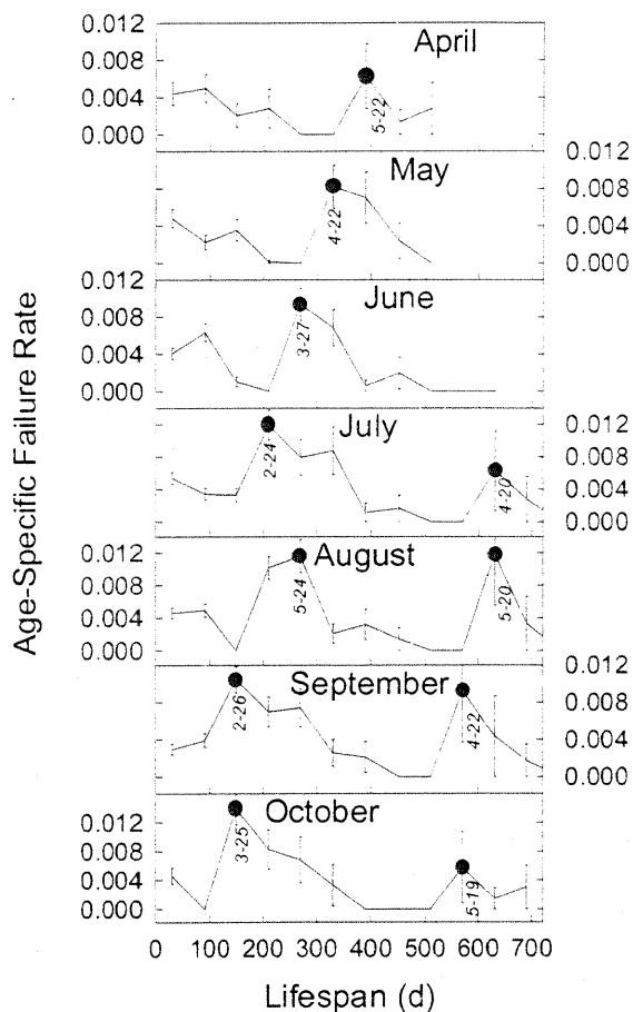
Figure 6. Estimated hazard functions versus lifespan for poplar roots stratified by month of appearance for the growing season. The hazard function is the probability that a root of a specific age will fail during the given time period (age-specific failure rate). All roots appearing during the specified month during the 1994–1996 observation period were included in the analysis. The appearance month is indicated with bold letters in each panel. Data are midpoints of the 60-day time interval. Symbols (●) mark peak hazard times for each appearance month. Numeric labels show peak hazard date. Error bars indicate the 95% confidence interval of the estimate.
