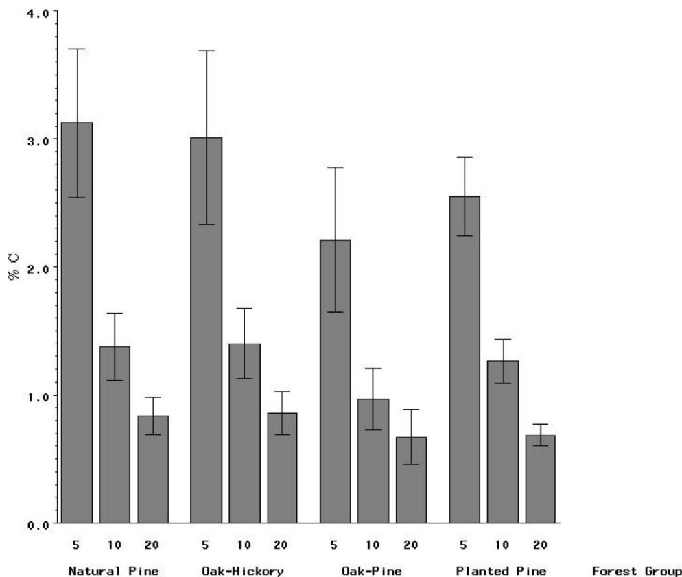
Fig. 8. Soil carbon concentration by forest group and depth increment (5 = 0–5, 10 = 5–10, and 20 = 10–20 cm).
