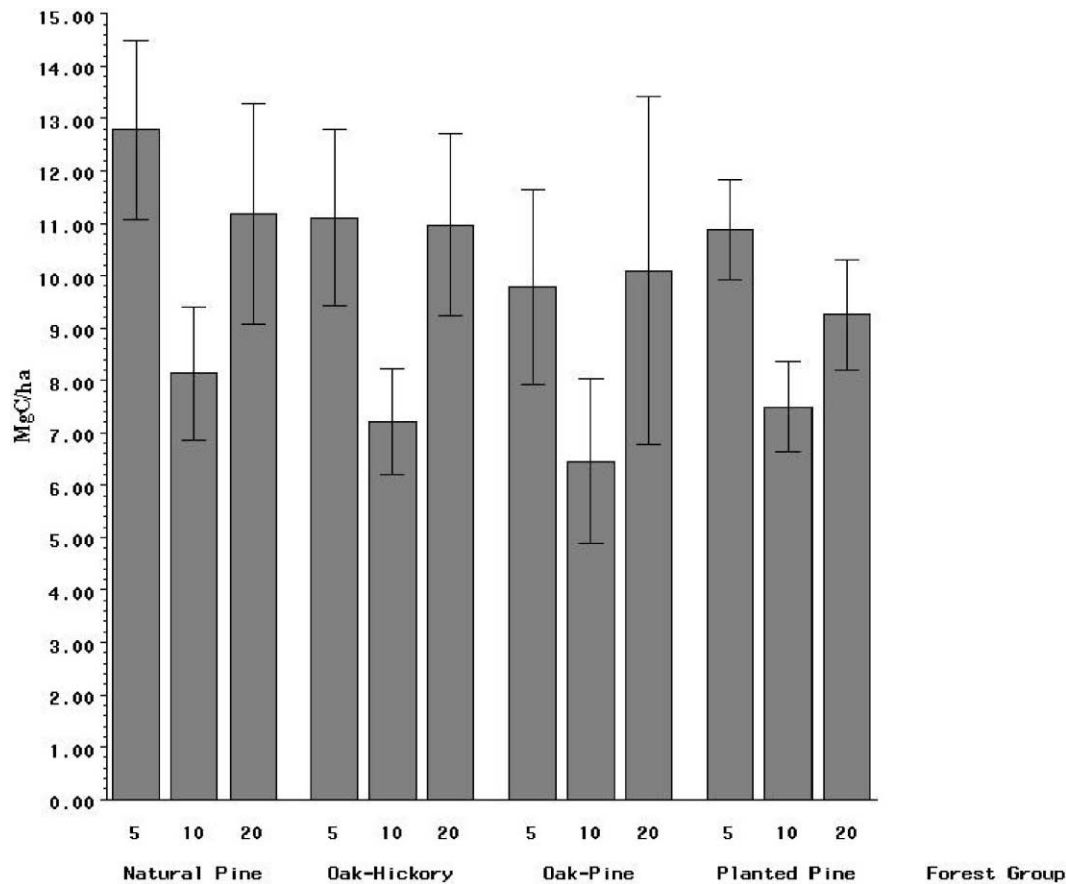
Fig. 9. Soil carbon content by forest group and depth increment (5=0–5, 10=5–10, and 20=10–20 cm). The number of plots included in each forest type was Natural Pine, 8; Oak–Hickory, 3; Oak–Pine, 3; Planted Pine, 16.
