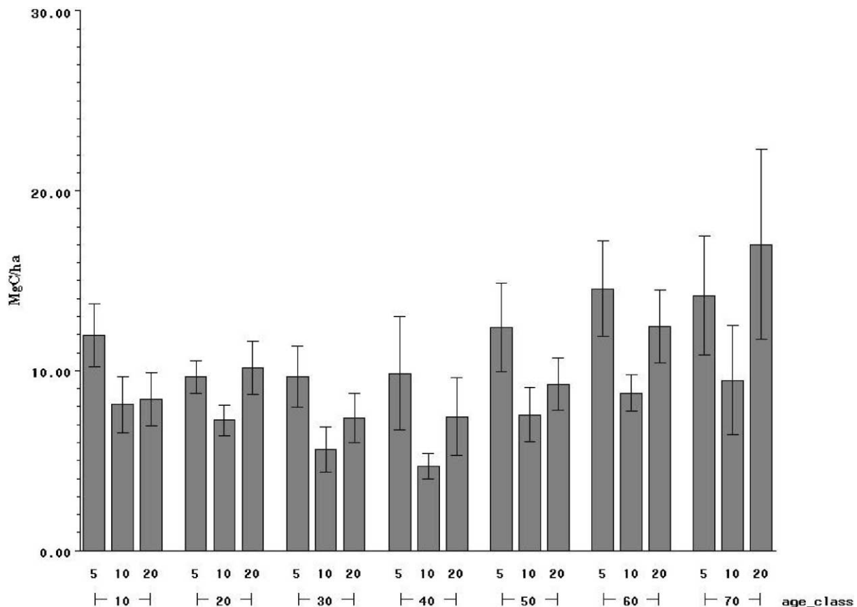
Fig. 10. Soil carbon content by age class (10=0–10 years, 20=11–20 years, 30=21–30 years, etc.) and depth increment (5=0–5, 10=5–10, and 20=10–20cm). The number of plots included in each age class was 0–10 (eight plots), 11–20 (nine plots), 21–30 (three plots), 31–40 (one plot), 41–50 (three plots), 51–60 (two plots), and 61–70 (three plots).
