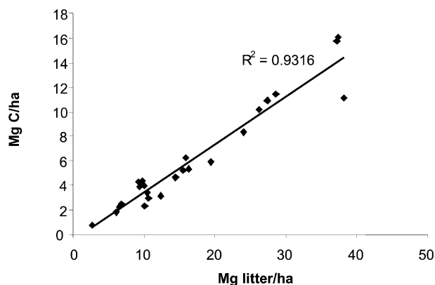
Fig. 5. Relationship between forest floor mass and forest floor carbon content.
