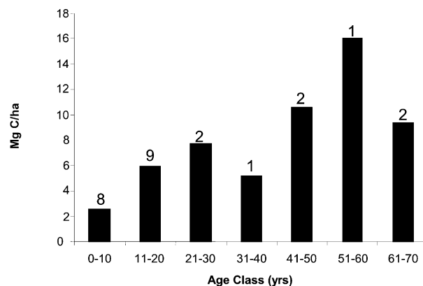
Fig. 4. Forest floor carbon by age class for pine and oak-pine plots. Numbers above bars indicate the number of plots included in the mean.
