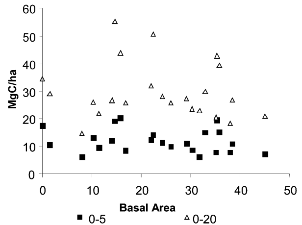
Fig. 7. Soil carbon content at two depths vs. basal area.
