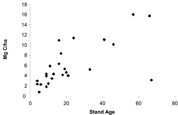
Fig. 6. Relationship between stand age and forest floor carbon content.
