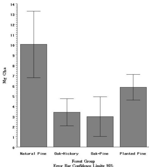
Fig. 2. Average carbon content of the forest floor by forest group.
