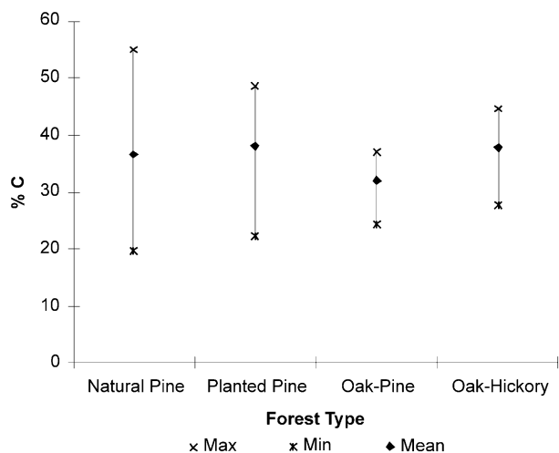
Fig. 3. Minimum, maximum, and mean C concentrations of forest floor material.
