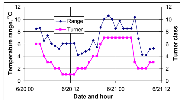
Fig. 6. The range of predicted temperature differences, \Delta T , and Turner Class across the map domain during a 32-h period on June 20 and 21, 2004 that were selected as representative of generally clear conditions near the solstice.
