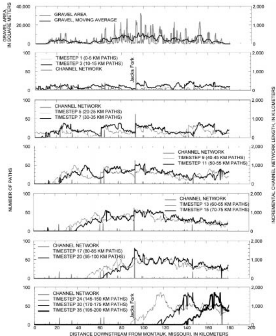
Figure 6.12—Longitudinal plots of gravel-bar area and moving average of gravel-bar area along the Current River (top graph) and results of a simple sediment routing model that depicts how uniform transport of sediment from first-order tributaries would merge downstream as wave-like forms. The distribution at timesteps 7 to 9 (corresponding to sediment traveling 30 to 45 km) replicates many of the features of the actual gravel-bar distribution. From Jacobson and Gran (1999).
