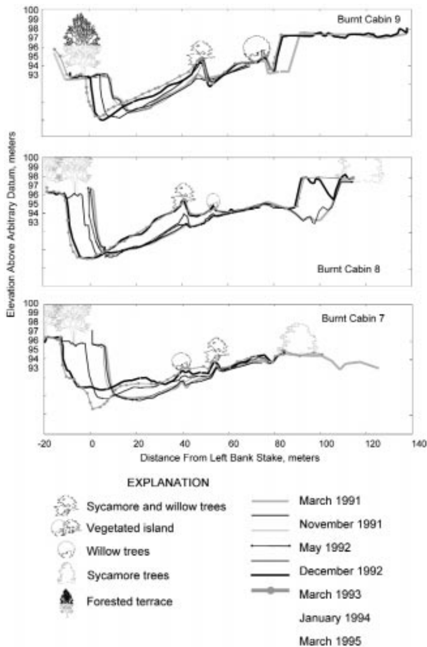
Figure 6.10—Channel cross sections at the Burnt Cabin reach showing the morphologic change during March 1991–March 1995. Trees on cutbank (to left) provide minimal resistance to erosion; trees growing on point bar (to right) trap sediment by providing hydraulic resistance. From McKenney (1997).
