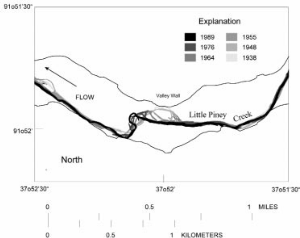
Figure 6.9—Record of channel changes in a dynamic stream system over 50 years, Little Piney Creek, Missouri. There are distinct longitudinal differences in inherent channel stability within the river segment. From Rabeni and Jacobson (1999).
