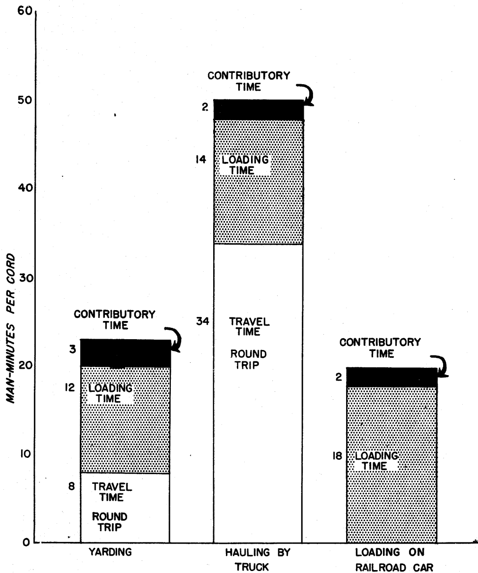
Figure 5.--Time consumed in transferring 4-foot aspen pulpwood from piles in the woods to railroad cars.
