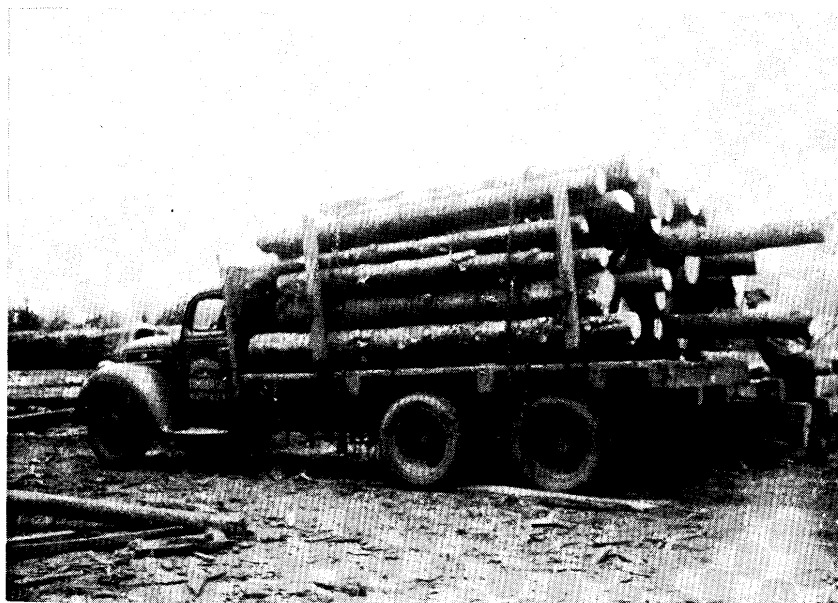
Figure 2.--A tandem-axle truck can haul about 2,000 board feet of logs per load.
