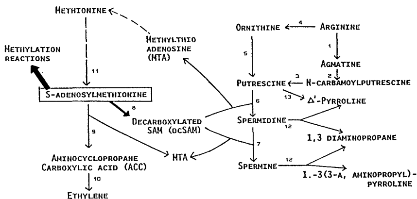
Figure 1. Combined pathway for biosynthesis of polyamines and ethylene in plants. The enzymes involved are: (1) arginine decarboxylase (ADC); (2) agmatine iminohydrolase; (3) N-carbamoylputrescine amidohydrolase; (4) arginase; (5) ornithine decarboxylase (ODC); (6) spermidine synthase; (7) spermine synthase; (8) SAM decarboxylase (SAMDC); (9) ACC synthase; (10) ethylene forming enzyme; (11) S-adenosylmethionine synthase; (12) polyamine oxidase (PAO); (13) diamine oxidase (DAO).
