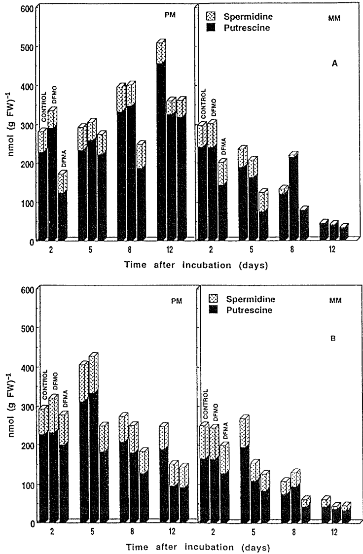
Figure 2. Effect of 2.0 mM DFMO and 0.1 mM DFMA on cellular levels of putrescine and spermidine in (A) Picea abies and (B) Picea rubens tissues grown on proliferation (PM) or maturation (MM) medium for different lengths of time. Values are mean \pm SE of 4 replicates for Picea abies and 3 replicates for Picea rubens . (Modified from Minocha et al. , 1993.)
