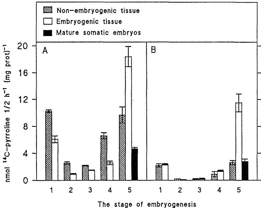
Figure 6. Activities of putrescine and spermidine oxidative enzymes in embryogenic and non-embryogenic tissues of P. abies (pH 8) during 5 stages of somatic embryogenesis in embryogenic tissue. At developmental stage 5, enzyme activity in somatic embryos and non-differentiated tissue were assayed separately. (A) DAO activity; (B) PAO activity. Values are mean \pm SE of three replicates. (Modified from Santanen and Simola, 1994.)
