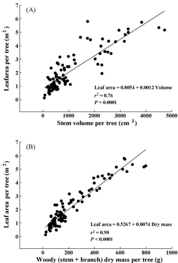
Fig. 3. Leaf area vs. stem volume (A) and woody (stem + branch) dry mass (B), per tree ( n = 100 for each).
