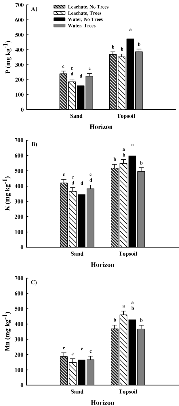
Figure 1 Concentration of P, K, and Mn for each combination of treatment (leachate and municipal water), cover (no trees and trees), and soil horizon (upper topsoil and lower sand) in tanks during an experiment testing clone-specific phytoremediation capabilities of Populus and Salix . Standard error bars represent one standard error of the mean, n = 3 trees for each three-way interaction, except for water and no trees where n = 1 . Concentrations with different letters above the bars are different according to Fisher's protected least significant difference (LSD) ( \alpha = 0.05 , LSD = 55.93 \text{ mg P kg}^{-1} , 73.99 \text{ mg K kg}^{-1} , and 76.03 \text{ mg Mn kg}^{-1} ).
