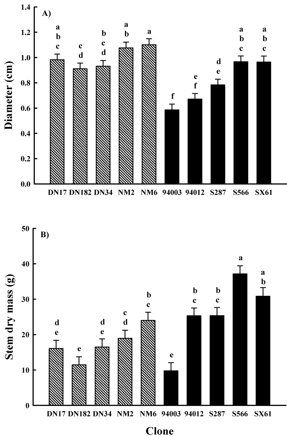
Figure 2 Diameter and stem dry mass across leachate and water treatments for Populus (dashed bars) and Salix (black shaded bars) clones during an experiment testing genotype-specific phytoremediation capabilities. Standard error bars represent one standard error of the mean, n = 12 trees for each clone. Traits with different letters above the bars are different according to Fisher's protected least significant difference (LSD) [ \alpha = 0.05 , LSD = 0.15 cm (diameter) and 7.48 g (stem dry mass)].
