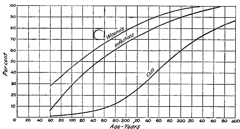
FIG. 3.—Relation of the age of incense-cedar trees to wounds, infections, and cull.
