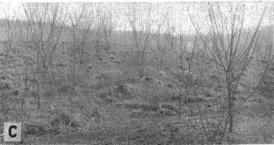
Figure 3.--These 4-year-old plantations on graded spoil banks in Fayette County, West Virginia, were planted in April 1946 by the New River Coal Company. A, red pine; B, white pine; C, black locust.
