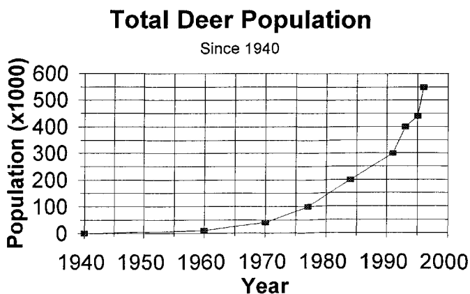
FIGURE 1. Estimated trends in deer populations in Ohio, 1940-1996.
