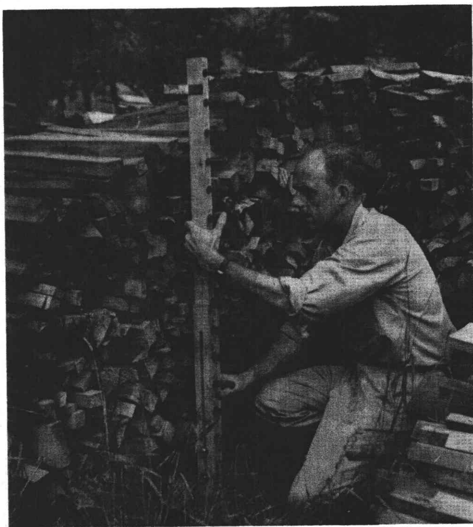
Figure 6.--Use of the special measuring stick for determining the percentages of wood and bark in a pile of slabs and edgings.
