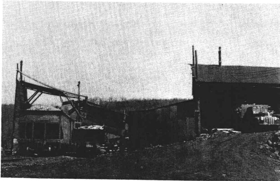
Figure 4.--New uses for slabs and edgings are being developed. At this railroad siding in Pennsylvania, slab material is made into chips for metallurgical uses. The material is brought to the chipping mill in pallets carried by a self-loading truck (right).
