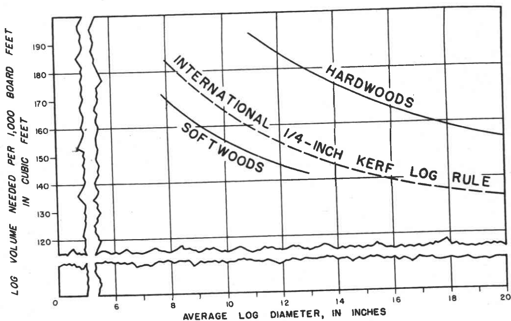
Figure 7.--The total cubic volume of logs needed by circular sawmills in Maryland to produce 1,000 board feet of lumber. This graph is based on cutting of lumber and dimension stock less than 4 inches thick.
