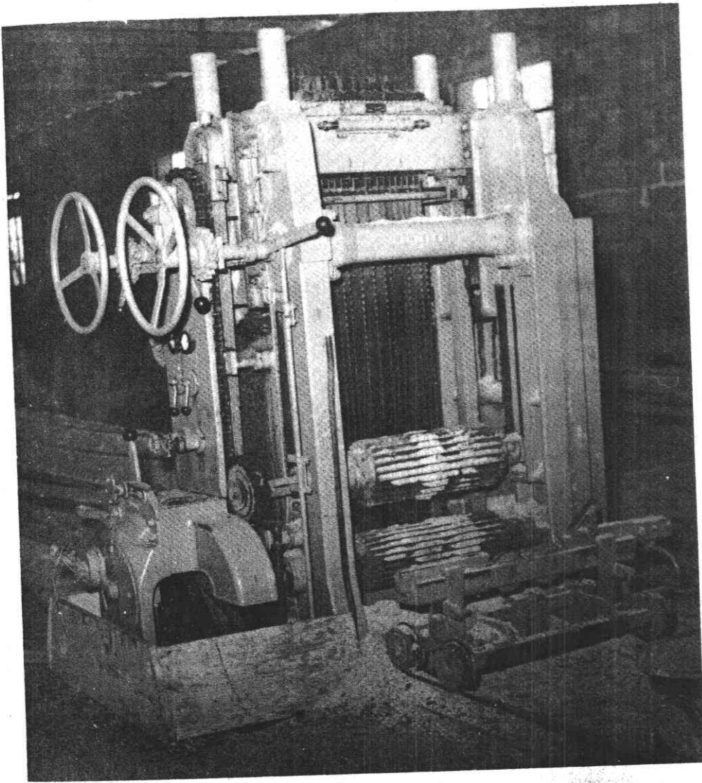
Figure 1.--A sash gang saw. This German-built machine is in use at a sawmill at Cocksackie, N.Y.
