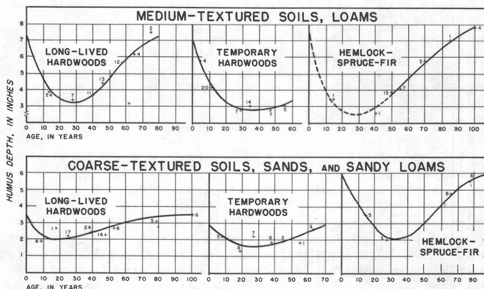
FIGURE 1.--Humus depth - age relationships. The numbered points indicate number of plots.
