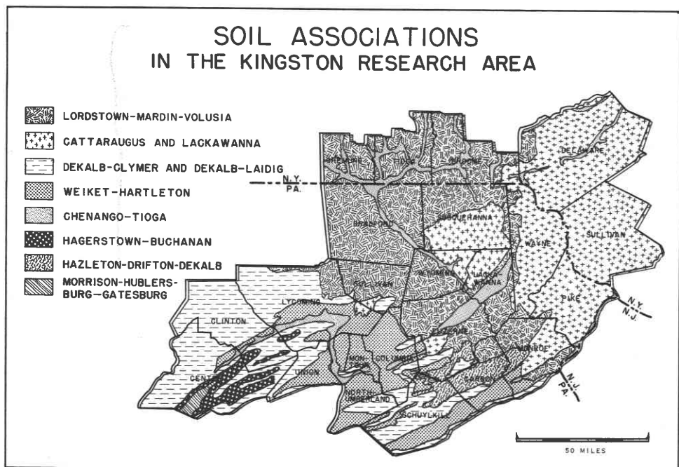
Figure 5.--General distribution of the soil associations in the Kingston Research Center area (15).
