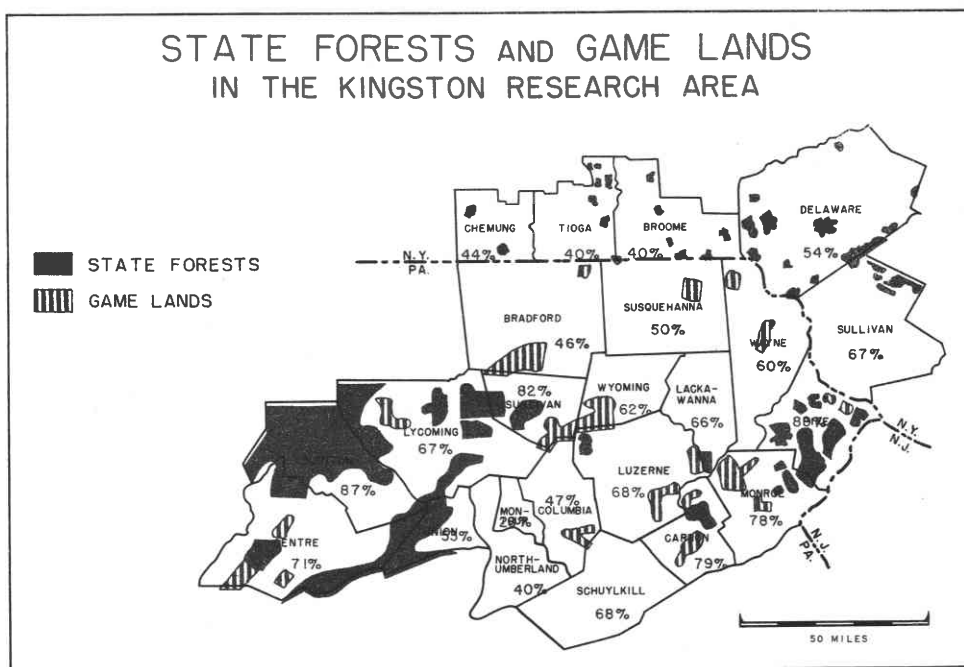
Figure 4.--Location of State Forests and Game Lands in the Kingston Research Center area. The percentage figures show how much of each county is covered by forest.
