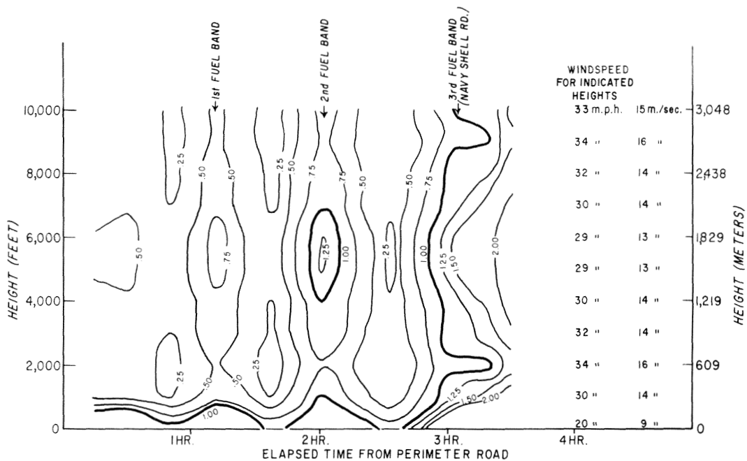
Figure 12. --Time-height cross section with isopleths connecting points of equal N_c value. These correspond to changes in fire intensity during the period when bands of unconsumed fuel were formed after the fire crossed Perimeter Road. An N_c value of 1 is depicted by the heavy isopleth lines.
