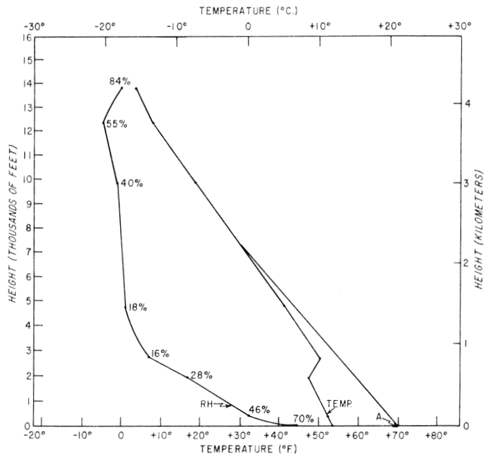
Figure 6.--Upper-air sounding taken at Cape Hatteras on March 22, 1971, at 0615 e.s.t. Point A indicates the surface temperature of 70° F. at 1100 e.s.t., and the line through this point depicts the temperature profile that would exist if the surface air was displaced vertically.
