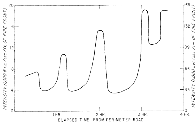
Figure 11. --Oscillations in fire intensity during the period when fuel bands were formed on Monday, March 22, after the fire crossed Perimeter Road.
