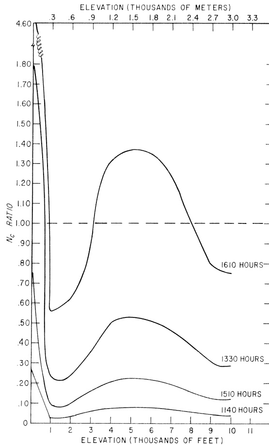
Figure 7.--Average N_C values at various heights and at four time intervals on Monday afternoon, March 22, 1971. Times indicated are the midpoints of selected periods from table 1.
