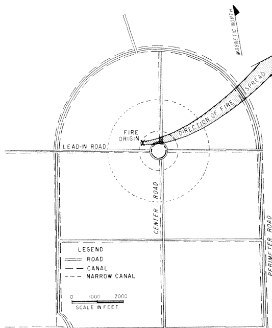
Figure 2.--The system of roads and canals used for access and fire control at the Dare County Air Force Bomb Range. Fire origin is marked by an "X."
