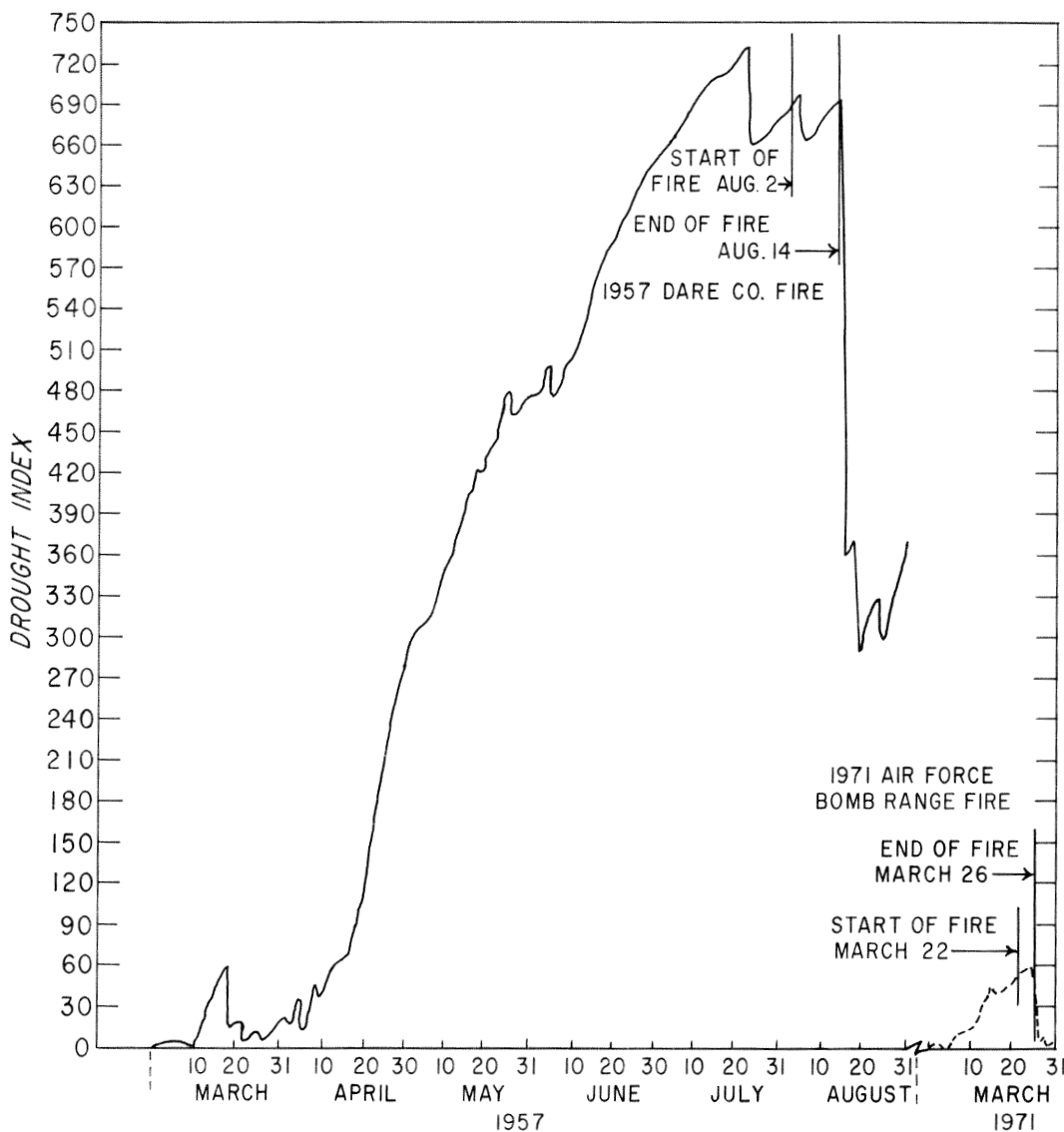
Figure 16. --Comparison of the 1957 and 1971 Drought Indices compiled from records at Elizabeth City, North Carolina.
