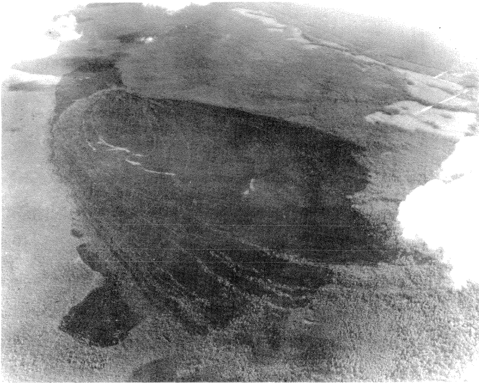
Figure 8. --Fuel patterns preserved on the Exotic Dancer Fire, which burned 2,000 acres (800 ha.) in eastern North Carolina on May 23, 1970. (Photograph by the North Carolina Forest Service.)
