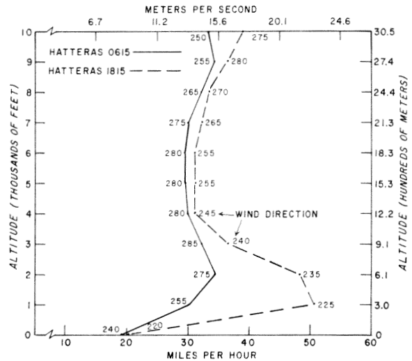
Figure 5.--Upper-air windspeed profiles at dawn and dusk of March 22, 1971, at Cape Hatteras. Wind direction is indicated by azimuth readings.
