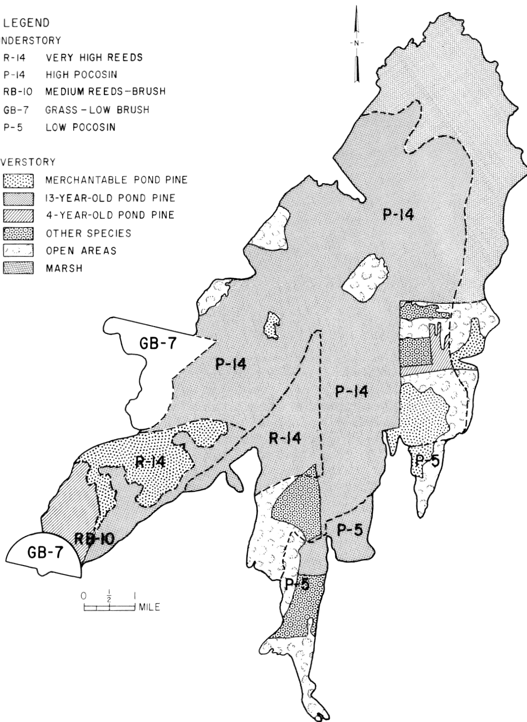
Figure 4.--Understory fuels and timber types on the burned area. [Understory map adapted from Wendel et al. (12). Overstory map adapted from: Honnold, Clark D. Damage appraisal, Westvaco Corporation lands, Dare County, North Carolina. 27 pp. 1971. (Appraisal rep., Appraisal contract DACA21-71-C-0071.)]
