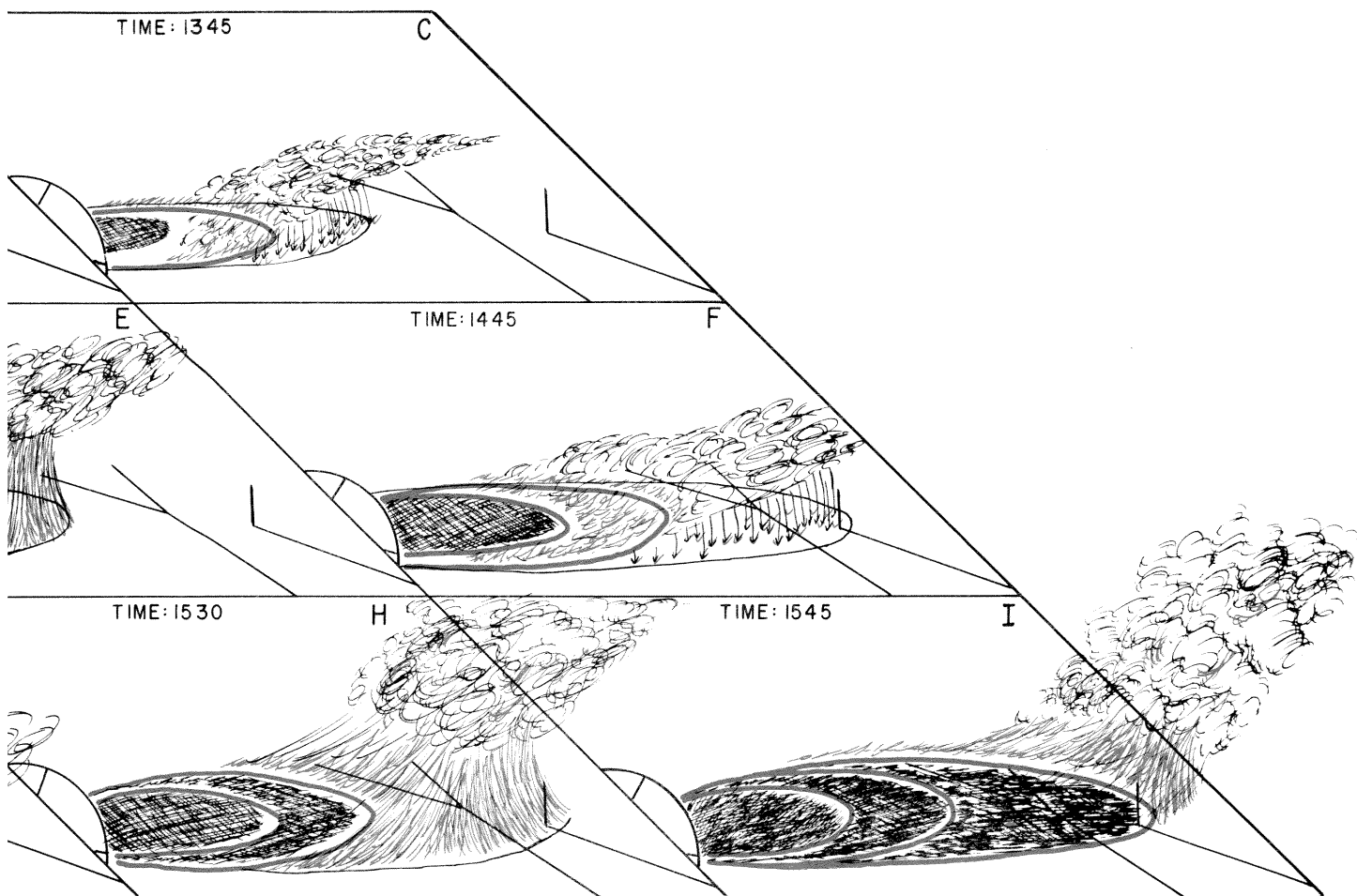
Figure 10.--Fire phenomena associated at various times with the formation of bands of unconsumed tree crowns as the fire progressed from Perimeter Road to Navy Shell Road. (See the text, page 23, for explanation of the drawings.)
