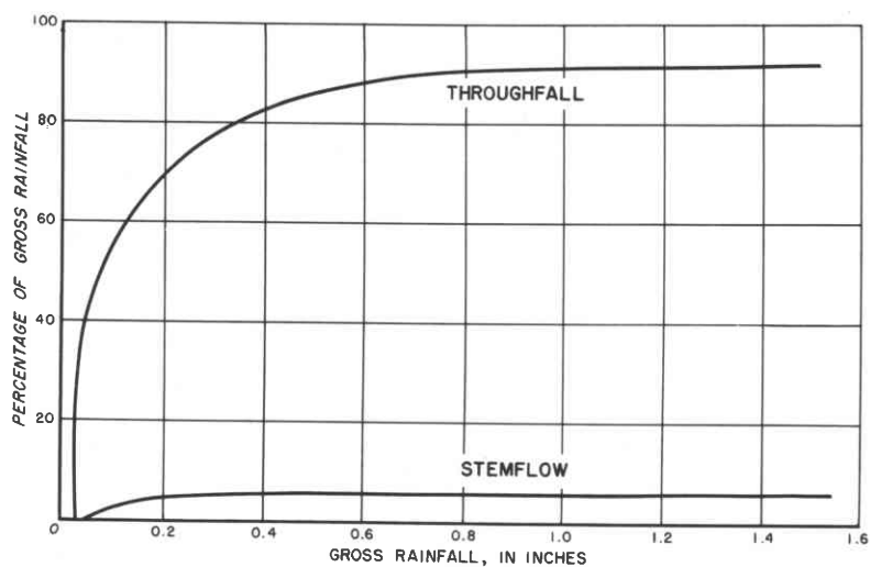
Figure 5. — Relationships between throughfall, stemflow, and gross rainfall.
