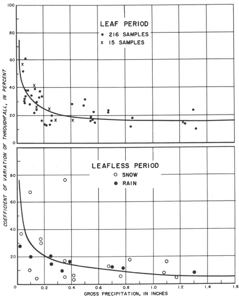
Figure 7. — The relationship of coefficient of variation of throughfall to storm size.
