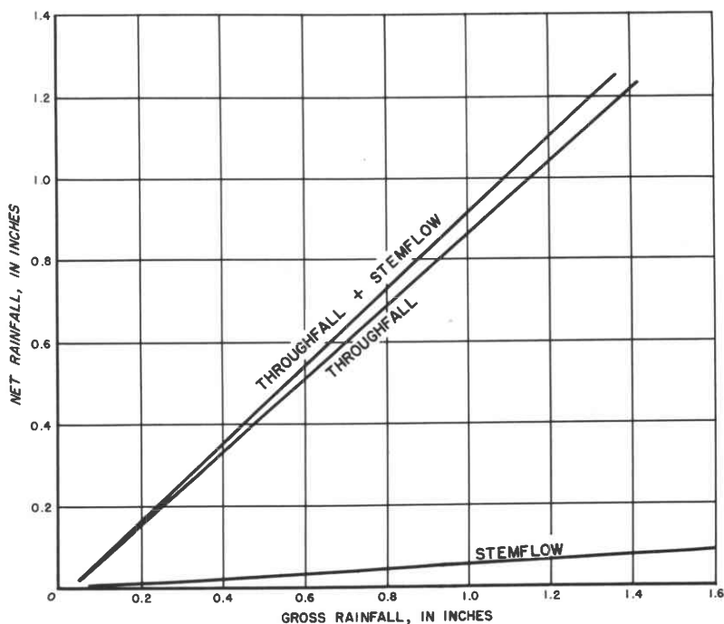
Figure 8. — The relationship between net rainfall (throughfall plus stemflow), throughfall, stemflow, and gross rainfall during the leaf period.
