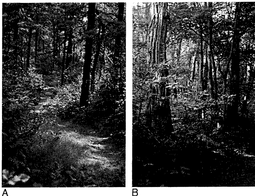
Figure 1. (a) Stand dominated by native, fire-adapted pitch pine, maintained using prescribed fire at the Albany Pine Bush in Albany, New York. (b) On a former agricultural field, sandy soils can become invaded by less flammable black locust, which is understood to be outside its native range north of Pennsylvania.
