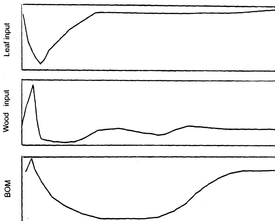
Figure 7.2 Hypothetical trends in allochthonous inputs and stream benthic organic matter (BOM) after riparian logging (modified from Hedin et al. 1988 and Webster et al. 1992).
