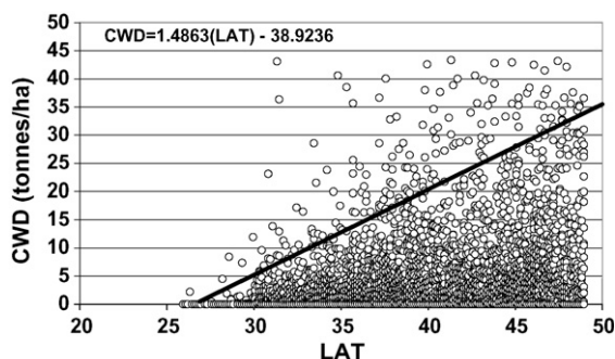
Fig. 1 – Coarse woody debris versus latitude including 97th percentile regression line for the U.S., 2001–2005.
