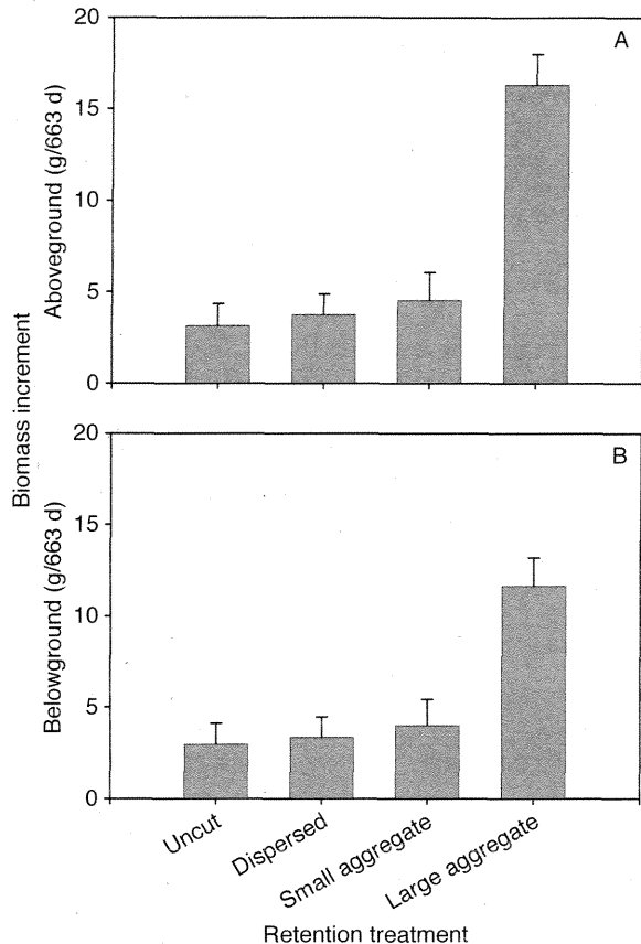
FIG. 8. (A) Aboveground and (B) belowground longleaf pine seedling biomass increment in four retention treatments in a longleaf pine woodland. Values are means \pm 1 SE of three replicates.
