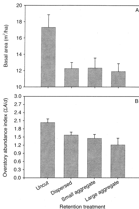
FIG. 3. (A) Overstory basal area and (B) overstory abundance index in four retention treatments in a longleaf pine woodland. Values are means \pm 1 SE of three replicates.
