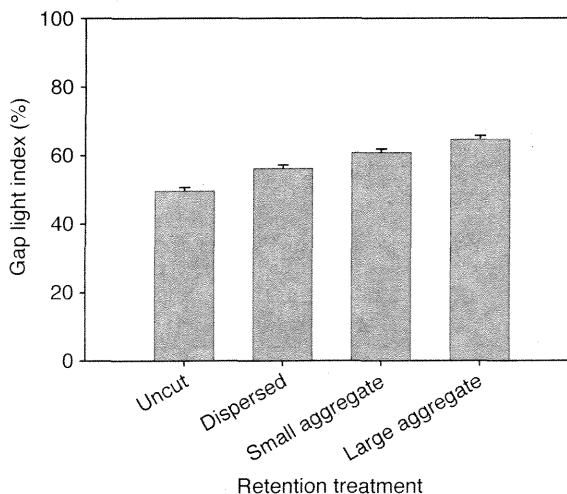
FIG. 5. Gap light index in four retention treatments in a longleaf pine woodland. Values are means \pm 1 SE of three replicates.
