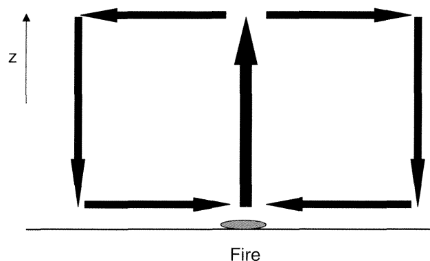
Fig. 2. Idealized, conceptual circulation of the atmosphere driven by fire with no environmental wind.
