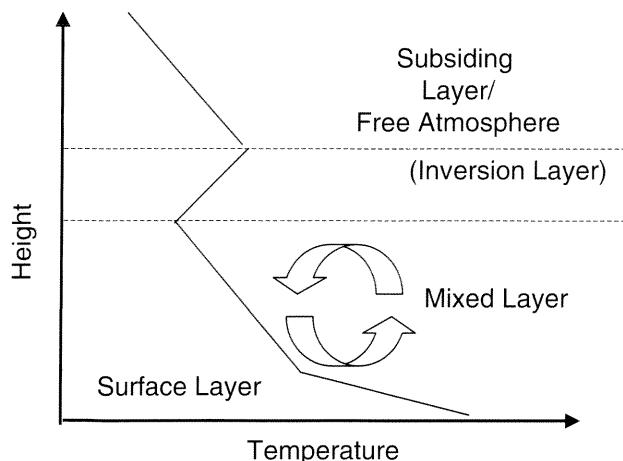
Fig. 1. Idealized vertical structure of the lower atmosphere.
