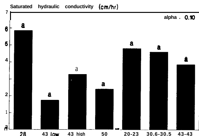
Figure 7. Average saturated hydraulic conductivity by tire width .
