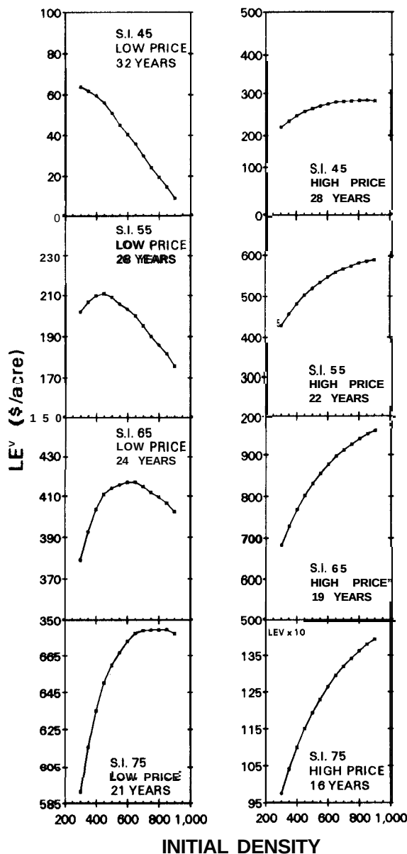
Figure 2. Planting density curves by site index for low and high pricing levels. YEARS refers to optimum rotation age.
