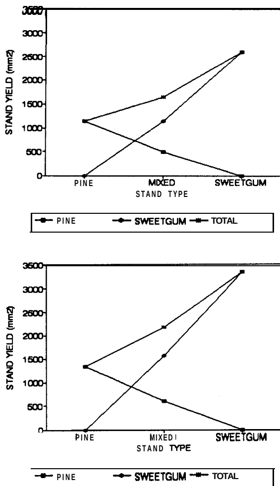
Figure 2. Relative yield for loblolly pine and sweetgum grown under low (350 ppm) (A) and high (800 ppm) (B) CO 2 in monoculture and pure stands. yield is presented in terms of volume per stand of 2.5 trees. For low CO 2 , RYT = .884 \pm .154 , RCCP = .986 \pm .154 , RCCS = .986 \pm .163 , RCCS = 1.04 \pm .180 . For high CO 2 , RYT = .913 \pm .150 , RCCP = 1.019 \pm .190 , RCCS = 1.008 \pm .191 .
