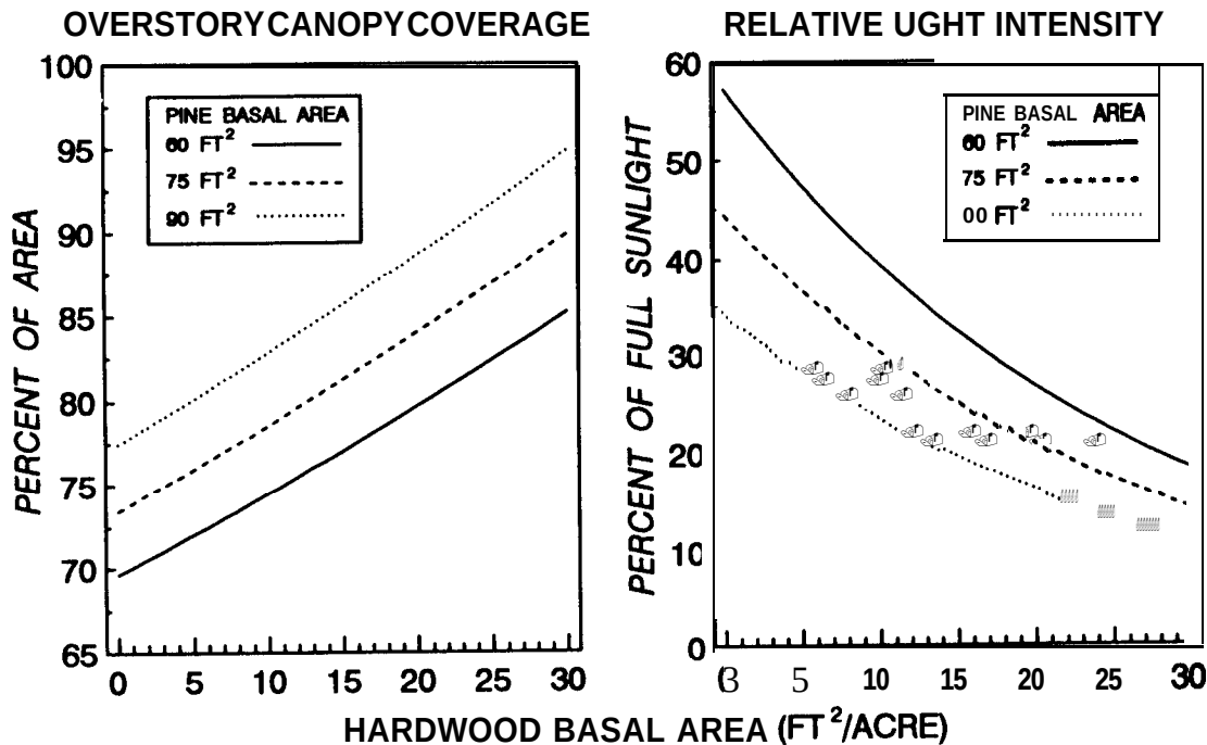
Figure 1. Effects of residual pine and hardwood basal areas on the overstory canopy coverage and relative light intensity 2 years after thinning a 35-year-old pine-hardwood stand.
