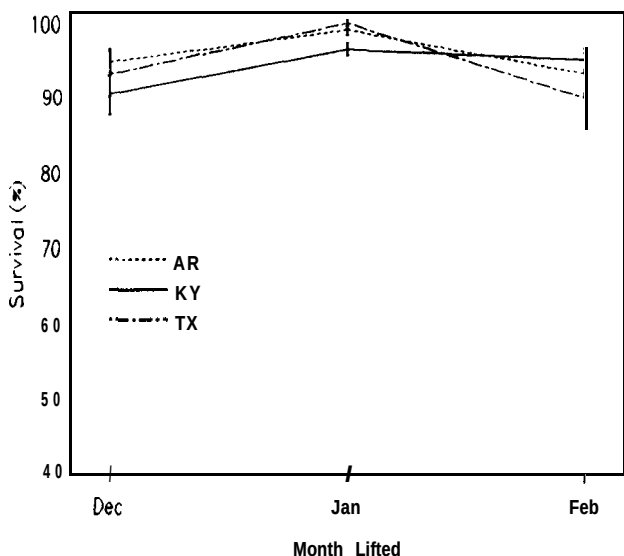
Figure 4. The interactive effect of seed source and lift date on the survival of shortleafpine seedlings grown at the USDA Forest Service W. W. Ashe Nursery. The vertical bars represent \pm 1 standard error of the mean.
