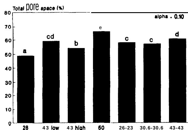
Figure 3. Average total pore space by tire width.
