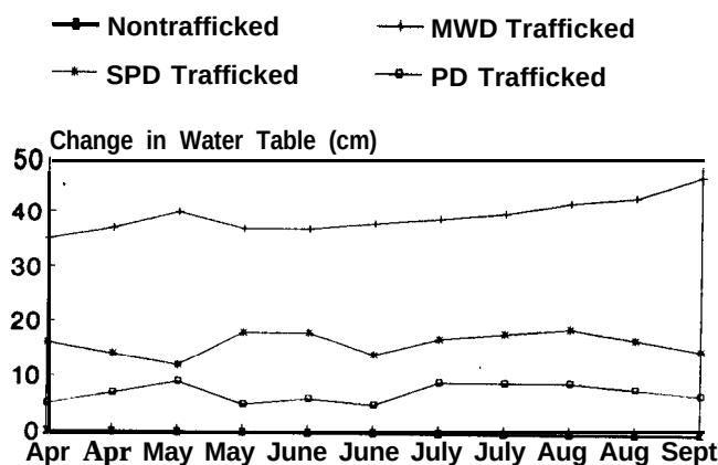
Figure 6. Relative response of water table to compaction .
