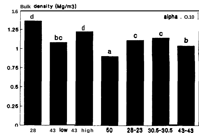
Figure 1. Average soil bulk density values by tire width.
