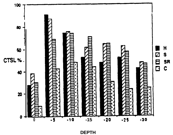
Figure 3. Cellulose decomposition - July 1992 (CTSL % = percent cellulose tensile strength loss, H = helicopter, S = skidder out of rut, SR = skidder in rut, C = control).
