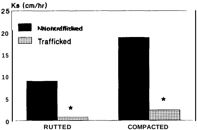
Figure 5. Average saturated hydraulic conductivity of rutted and compacted sites.
