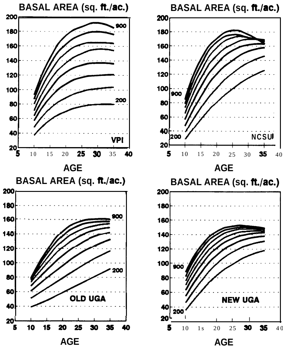
Figure 3. Basal area growth curves for various initial densities on site index 60 (Base-age 25) land for various growth and yield models.
