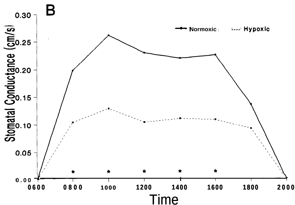
Figure 3. (A) Diurnal transpiration and (B) stomatal conductance for four species of bottomland oak seedlings during 35 days of rhizosphere hypoxia. Significant differences ( \alpha = 0.05 ) between dissolved oxygen treatments are noted by an asterisk above the x-axis.
