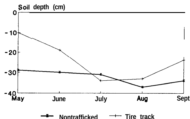
Figure 8. Effect of rutting on depth of rust on steel rods.
