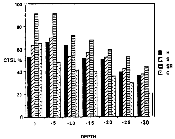
Figure 4. Cellulose decomposition - August 1992 (CTSL % = percent cellulose tensile strength loss, H = helicopter, S = skidder out of rut, SR = skidder in rut, C = control).
