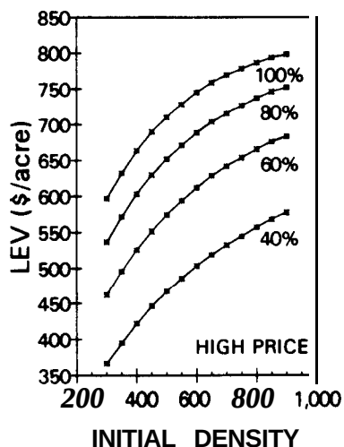
Figure 6. Planting density curves by initial survival for low and high pricing levels.
