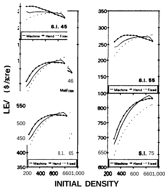
Figure 5. Planting density curves by site index for fixed and variable hand and machine planting costs.
