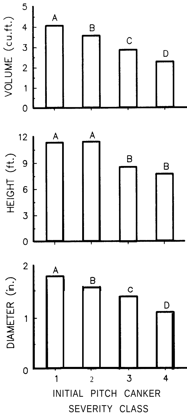
Figure 2. Adjusted mean, post-thinning 5-year growth for slash pines of four different initial levels of pitch canker-induced crown loss severity. Pitch canker (PC) severity class 1 = no loss, healthy; 2 = Trace-1096 crown loss; 3 = 11-30% crown loss; 4 = 31-50% crown loss. Within each graph, means from adjacent classes (1 vs 2, 2 vs 3, 3 vs 4) with a common letter do not differ significantly ( p = 0.05 ) according to least-squares means t-tests.
