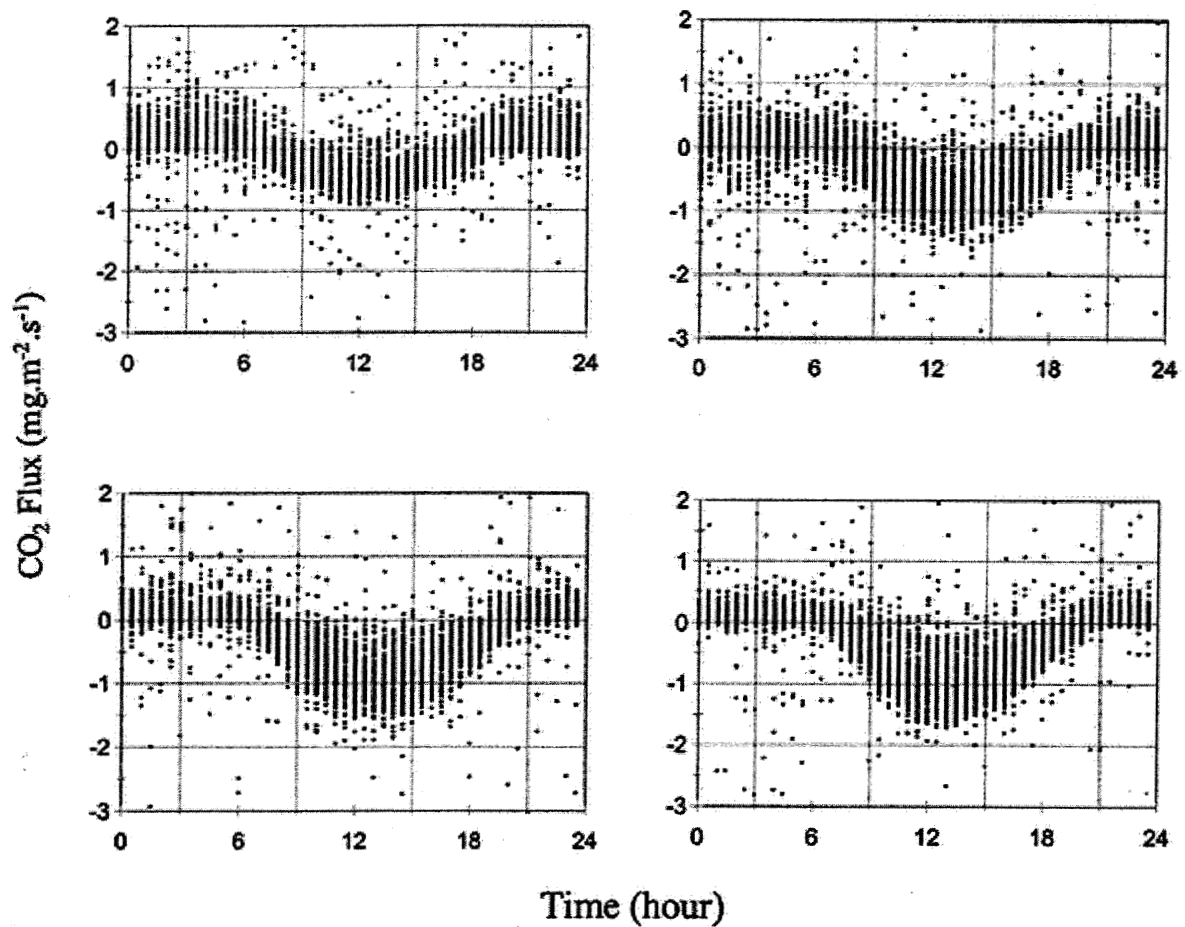
Figure 4 Diurnal patterns of net exchange of \text{CO}_2 (30-min means) in young and mature hardwood and conifer forests (i.e., two dominant ecosystem types) in the Chequamegon National Forest, Wisconsin, USA Data were calculated based on eddy-covariance measurements at four canopy-access towers. Negative values indicate carbon assimilation (i.e., net carbon gain) and positive values indicate net carbon loss.
