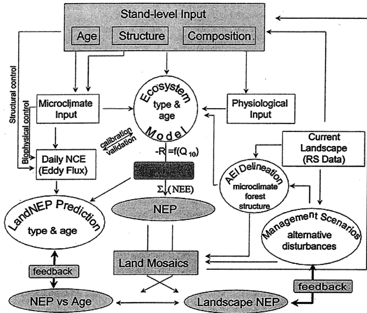
Figure 1 Conceptual framework for studying landscape-level carbon flux and storage in disturbed land mosaics, with explicit consideration of disturbance regime and landscape structure, including the area-of-edge influences (AEI).
