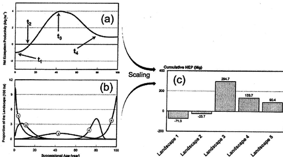
Figure 3 Hypothesized changes in net ecosystem production (NEP) with developmental age in a particular ecosystem (a) acts in concert with the age structure of the landscape (b) to determine the cumulative NEP of the landscape (c). In (a), t_1 – t_4 identify four different time periods along the developmental spectrum for comparison. In (b), the age
