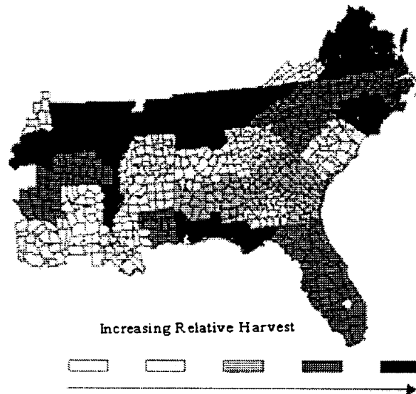
Figure 10 Predicted southern pine harvest shifts within each FIA survey unit from 1990 to 2040 across the southern US.
