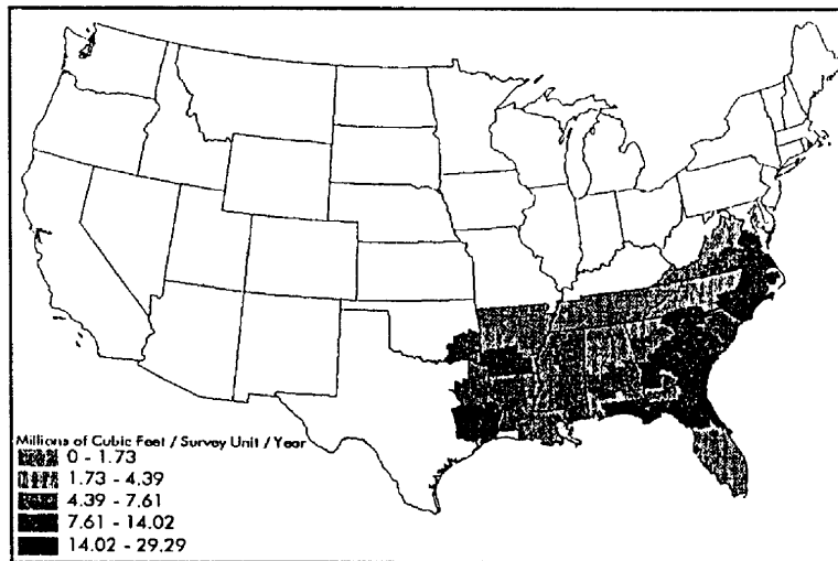
Figure 7 Predicted annual forest growth within each FIA survey unit between 2035 and 2045.
