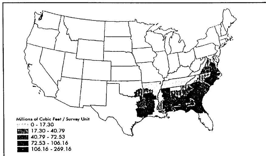
Figure 2 Measured FIA southern pine volume across the 51 southern US survey units.
