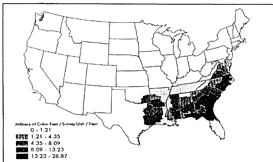
Figure 3 Measured FIA southern pine forest growth across the 51 southern US FIA survey units.
