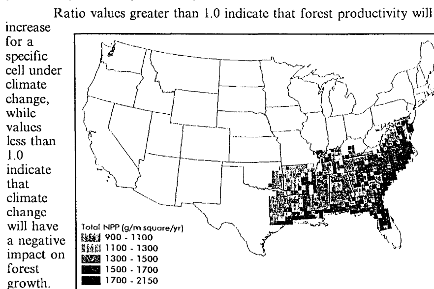
Figure 5 Predicted southern pine distribution and NPP in 2040 using the Hadley2sul climate scenario on a 0.5^\circ x 0.5^\circ grid.
