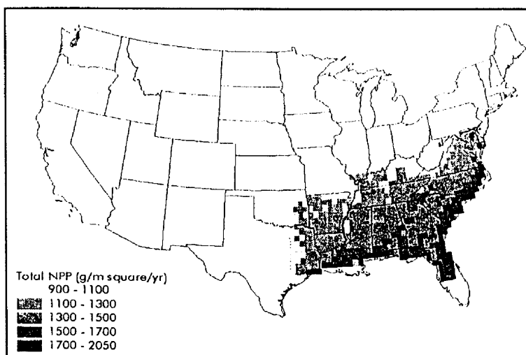
Figure 4 Predicted historic southern pine distribution and NPP on a 0.5^\circ \times 0.5^\circ grid.
