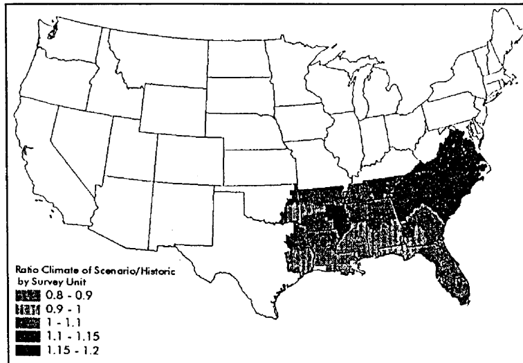
Figure 6 Predicted ratio of historic and climate scenario NPP between 2000 and 2040 regrided onto the 51 southern US FIA survey units.
