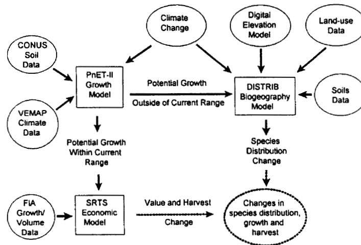
Figure 1 Linked forest process, biogeography, economic model structure.
