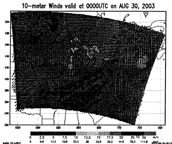
Figure 2. EMAC map of 10-meter Wind (meters/sec) at 12km resolution initialized at 0000 August 29, 2003, 24 hours after model initialization.
