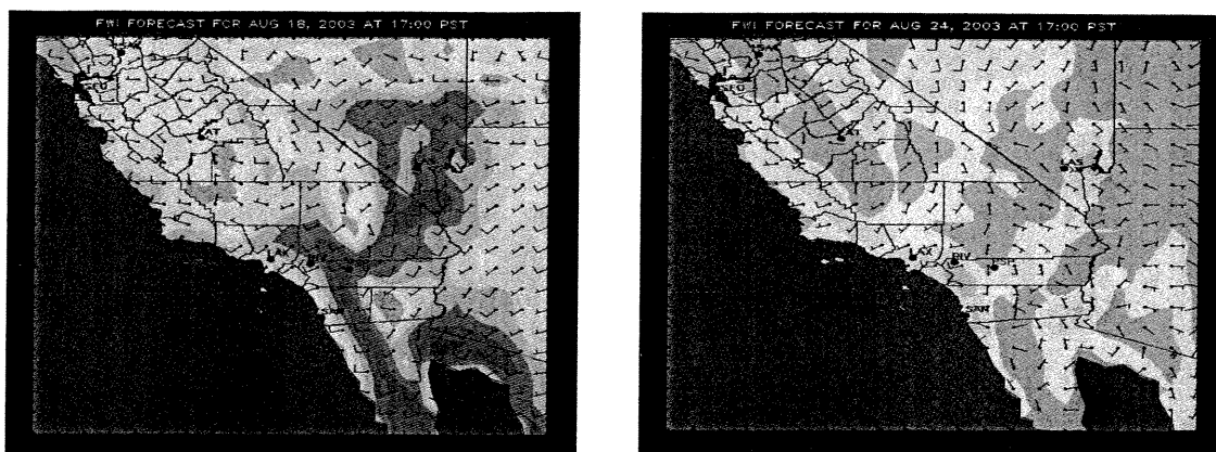
Figure 6. California Fire Weather Index (red as highest index value), produced by the California Smoke and Air Consortium in collaboration with Scripps Institute. The forecast is for 7 days, illustrated as a 24-hour forecast at 17:00 August 18 and 168 hour forecast at 17:00 for August 24.
