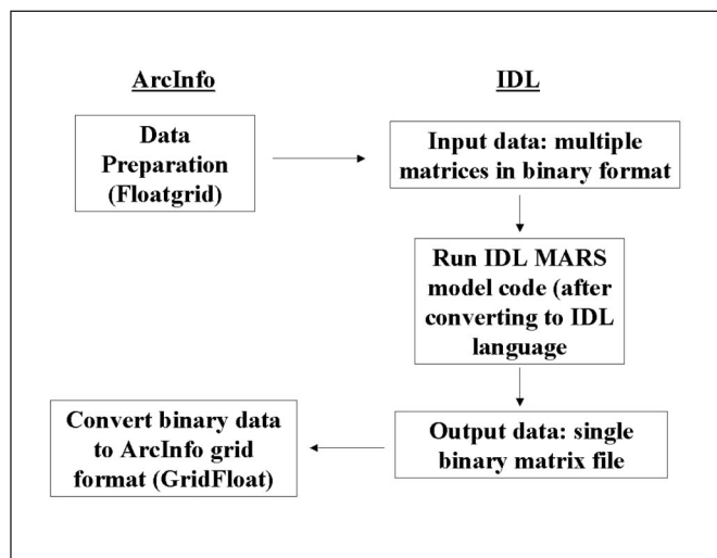
Figure 3.—Process of implementing a spatially explicit model in IDL.
