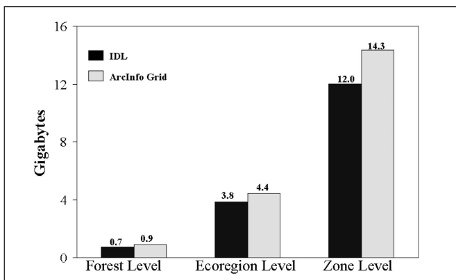
Figure 6.—Comparison of required storage for the simple model in the ARCINFO and the IDL software packages.
