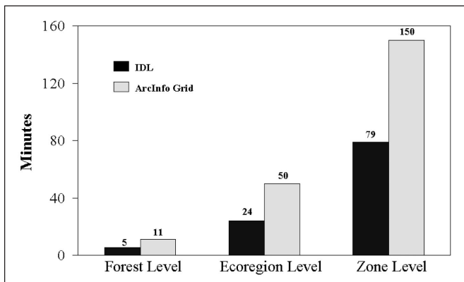
Figure 4.—Comparison of the time it took to run a simple mode (6 inputs, 13 intermediate grids (binary data for IDL), and one output) for three levels in the ARCINFO and the IDL software packages.
