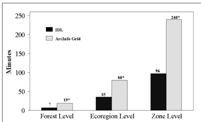
Figure 5.—Comparison of the time it took to run a complex model (9 inputs, 20 intermediate grids (binary data for IDL) and one output) for three levels in the ARCINFO and the IDL software packages.
