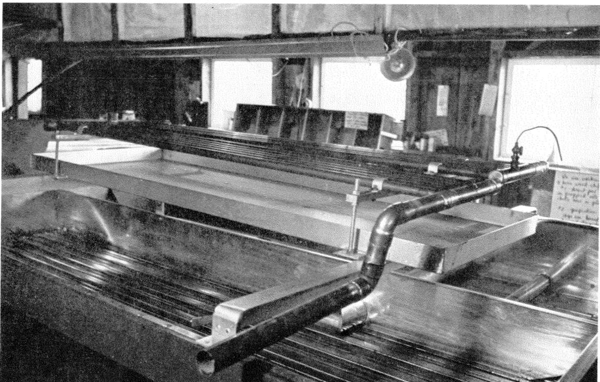
Figure 3.—Experimental parallel flow heat exchanger designed for a 4- by 6-foot flue pan.
