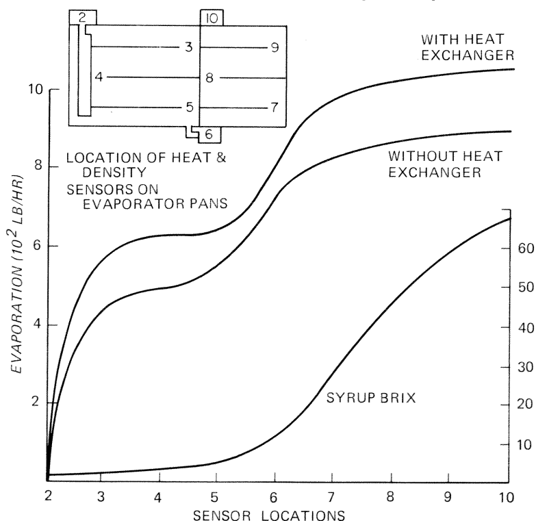
Figure 4.—Total accumulative evaporation and syrup Brix level at different locations in evaporator pan.
