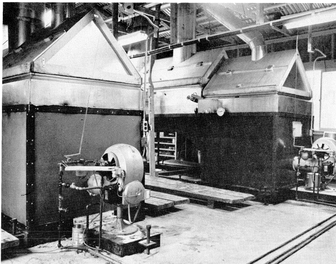
Figure 1.—Identical 4- by 10-foot Grimm evaporators used in lab tests to determine efficiency with and without a heat exchanger.
