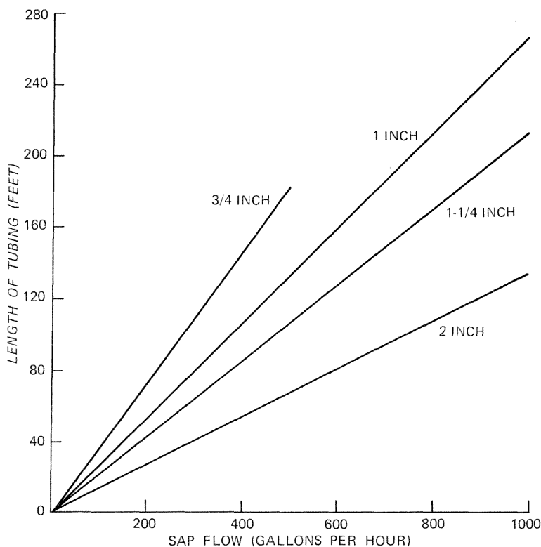
Figure 5.—Length of tubing required for parallel flow heat exchangers using different tube diameters at different flow rates.
