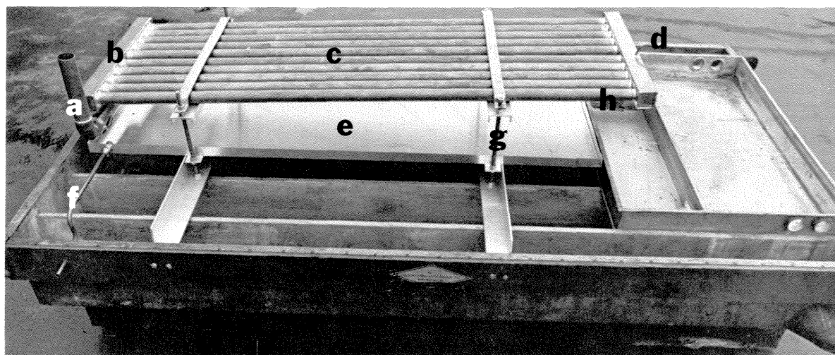
Figure 6.—A commercial design of the parallel flow heat exchanger design show: a) Sap inlet; b) Connector manifold; c) Tube bundle; d) Pressure release tube; e) Drip pan; f) Drip pan drain; g) elevating rods; h) Sap outlet.
