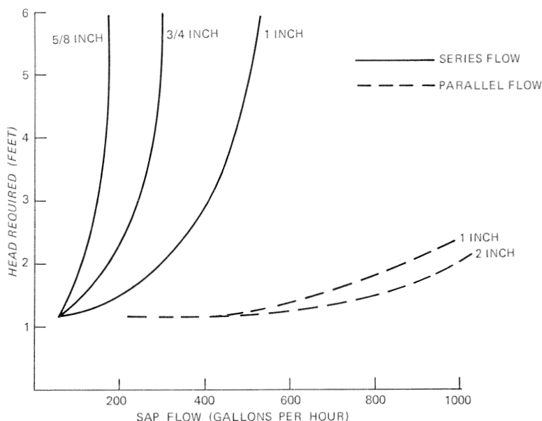
Figure 7.—Head requirements for series and parallel flow heat exchangers using different tube diameters.
