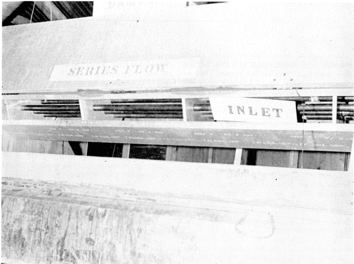
Figure 2.—Series flow heat exchanger designed for a 4- by 6-foot flue pan.
