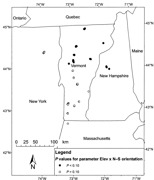
Fig. 4. The effect of elevation \times N-S orientation on 2003 red spruce winter injury from the GWR local models (model 3). Although the Student's t test for any one plot is statistically valid for that individual local regression model, no correction has been made for group-wise error. As a result, this map should not be used to determine precisely where this parameter was significantly nonzero. However, because P values less than 0.10 (filled plot circles) are concentrated in the northern portion of the study area, this map does provide an indication of the general area for which this parameter was important for accounting for winter injury patterns. Many plots overlap when viewed at this scale.
