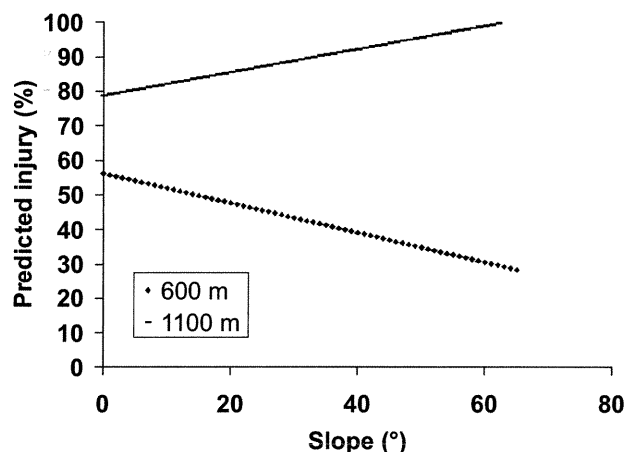
Fig. 3. Predicted injury versus slope plotted at two elevations to illustrate the effect of the interaction between elevation and slope in GWR's global model (model 2) on 2003 red spruce winter injury in Vermont and surrounding states.
