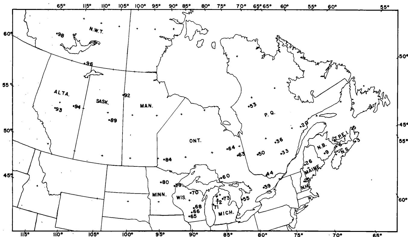
FIGURE 1. — Location of the 34 jack pine seed sources used in the measurement of tracheid length and specific gravity.
