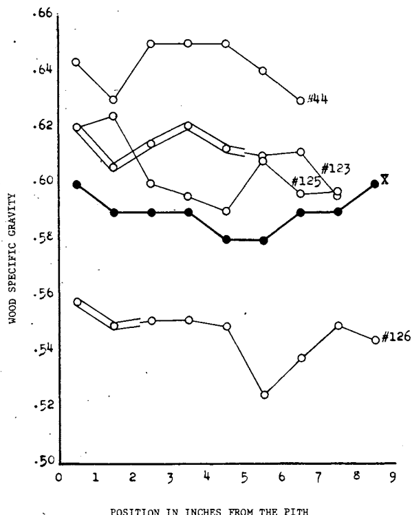
FIGURE 8. — Variation in specific gravity at breast height in relation to position for the average of all trees and for four selected individual trees. The double lines indicate the amount of heartwood.
