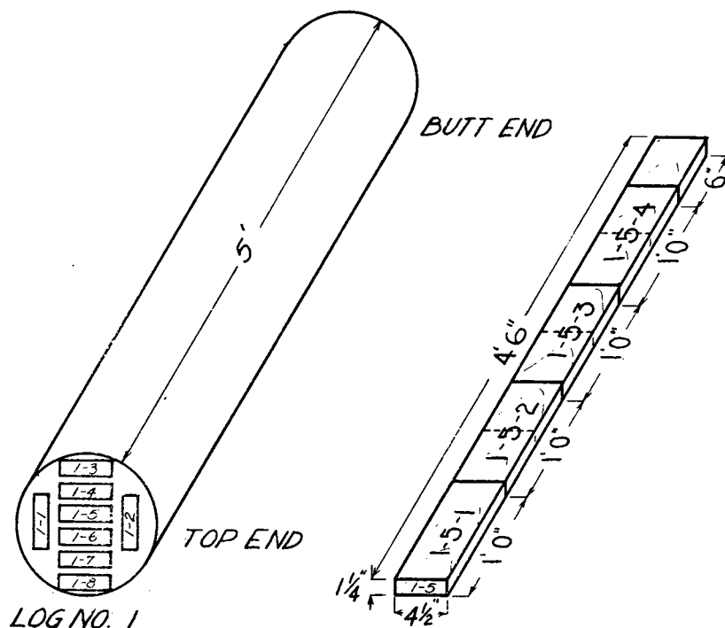
FIGURE 2. — Location of and numbering sequence for 1-foot samples in the boards.
