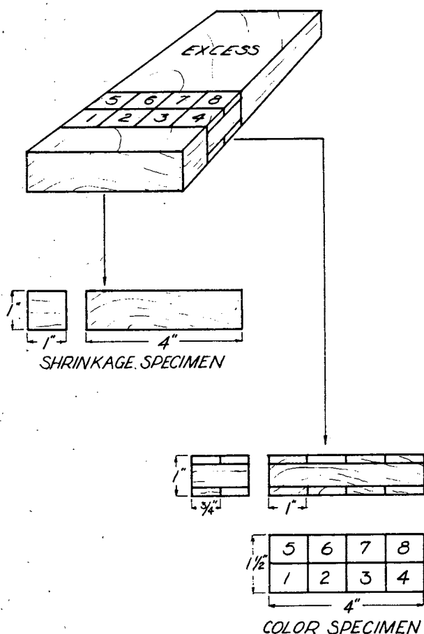
FIGURE 3. — Location of and numbering sequence showing shrinkage and color specimens.
