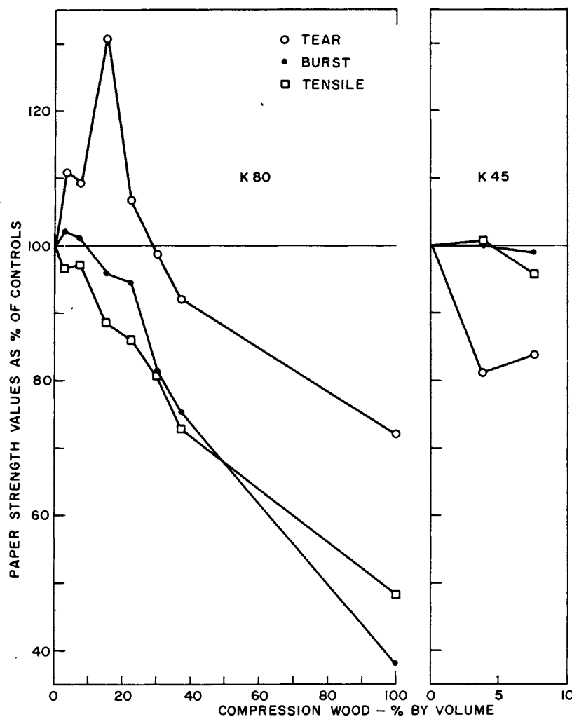
FIGURE 6. — Compression wood and paper strength values expressed as a percentage of the control values.
