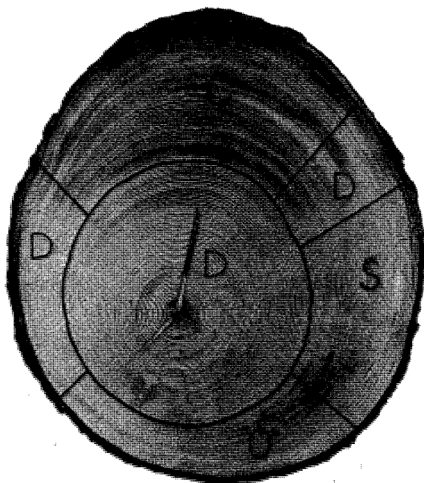
FIGURE 4. — Delineation of discs for pulp and paper-making tests. C is taken to be 100-percent compression wood. S (sidewood) and O (opposite wood) are taken as no compression wood; these were combined to give "normal" or control fraction. D is discarded as containing varying amounts of compression wood.
