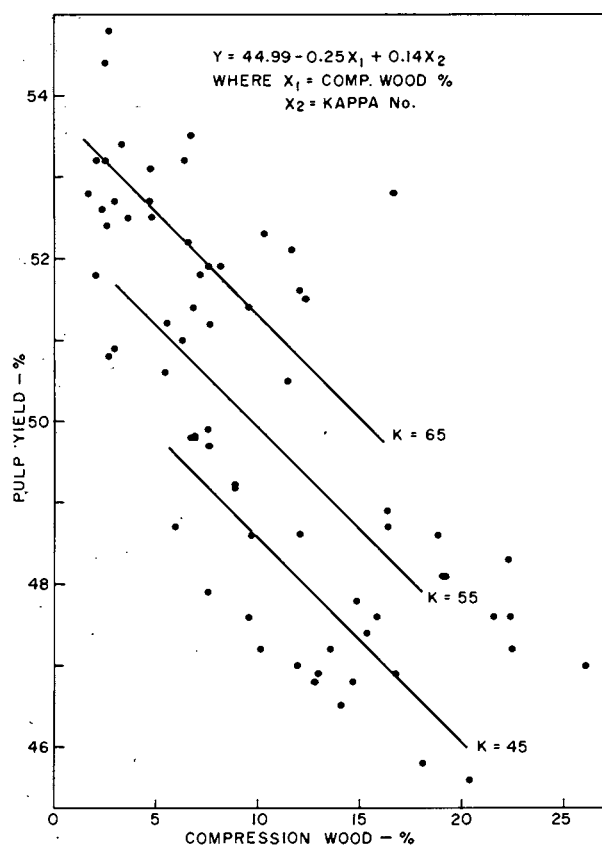
FIGURE 3. — Pulp yield and compression wood for pulps cooked to different lignin contents.
