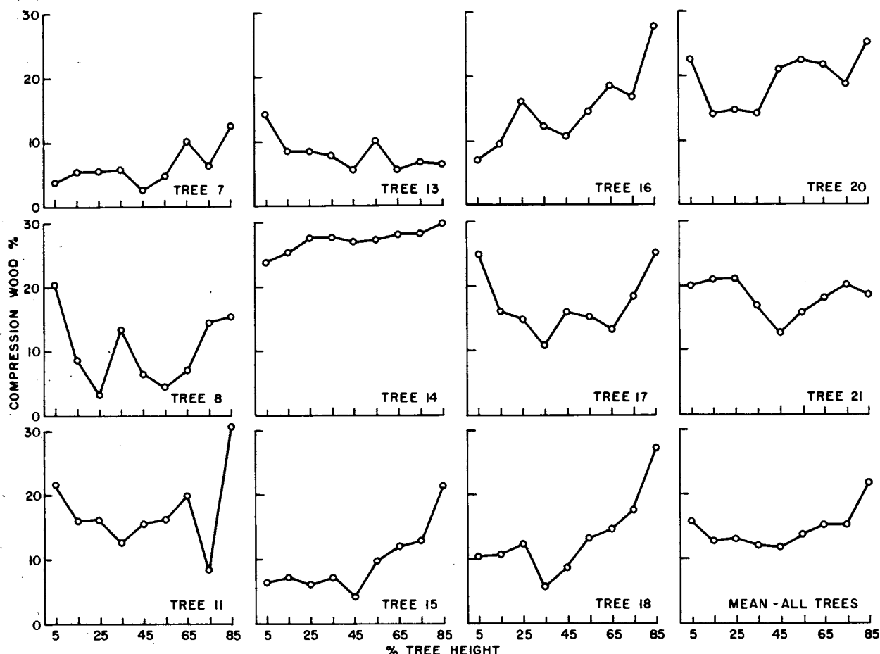
FIGURE 1. — Variation of compression wood content with height in each of 11 black spruce trees and in all trees combined.
