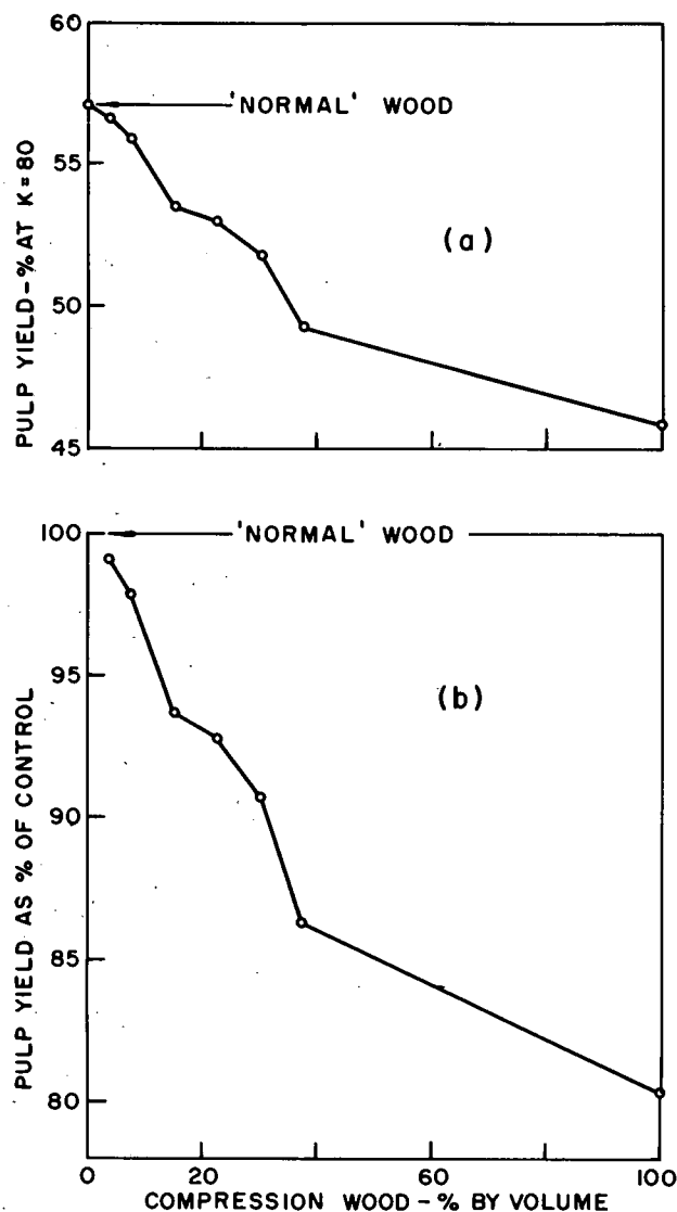
FIGURE 7. — (a) Compression wood content and screened pulp yield; (b) compression wood content and screened pulp yield expressed as a percentage of the yield from "normal" wood.
