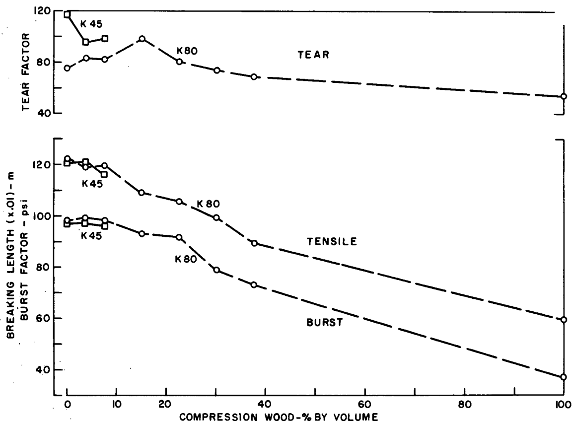
FIGURE 5. — Compression wood content and paper strength.
