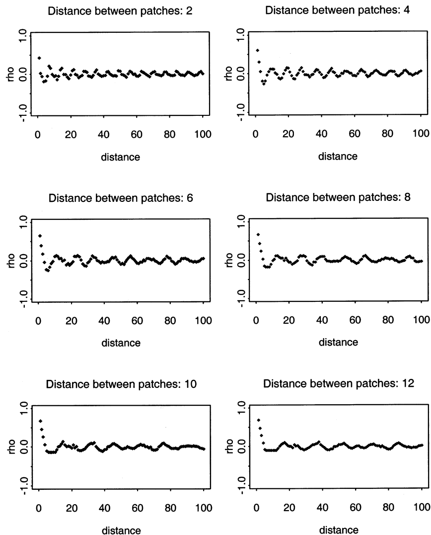
Fig. 7. Effect of changing distances between patch centers in a grid (Fig. 1b) with patch size being constant.
