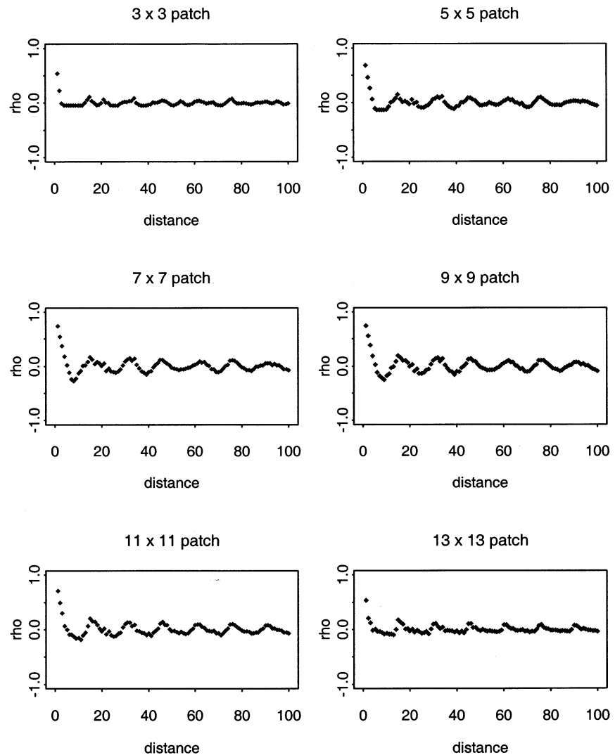
Fig. 6. Effect of changing patch size in a grid (Fig. 1b) with distance between patch centers being constant.
