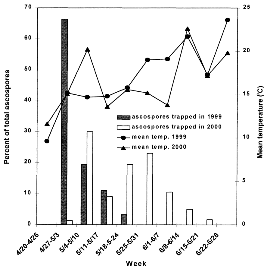
Fig. 1. Percentage of total Apioplagiostoma populi ascospores trapped versus mean weekly temperature in 1999 and 2000. Spore traps were changed weekly during 1999 and 2000. The total number of spores was tallied, and the number counted each week is represented as a percentage of the total for the year. Temperature data are taken from a weather station located approximately 0.8 km from the study site.
