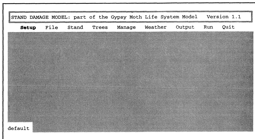
Figure 2. Main menu.
