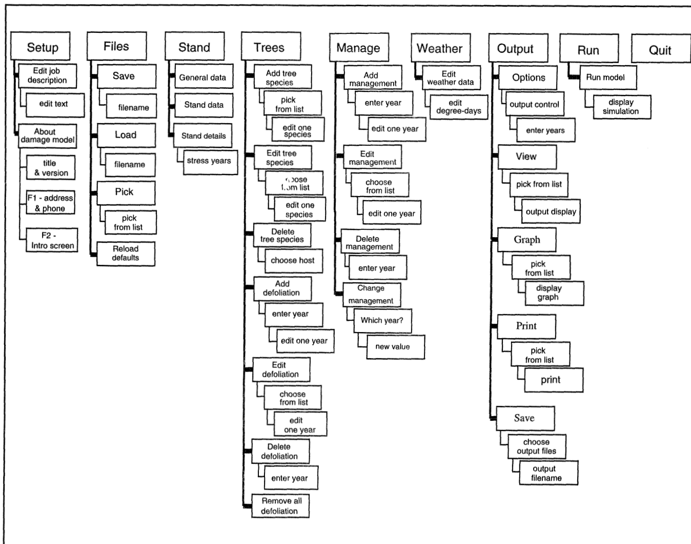
Figure 17. Structure of the menus and subordinate screens and windows.
