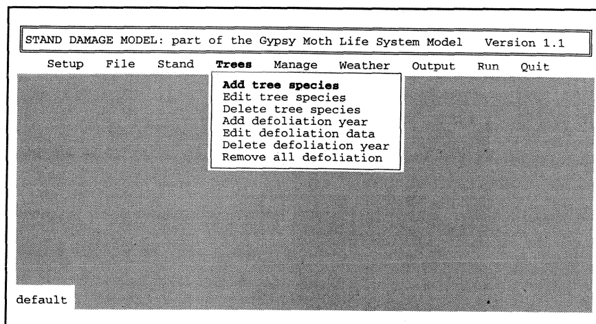
Figure 3. The Trees pull-down menu provides access to add, edit, or delete tree species-specific data, including defoliation by canopy strata within species.
