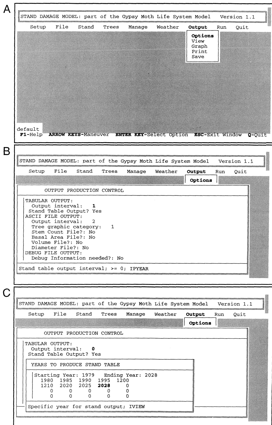
Figure 7. (A) Output pull-down showing submenus; (B) Options activated; (C) Output interval edit window.
