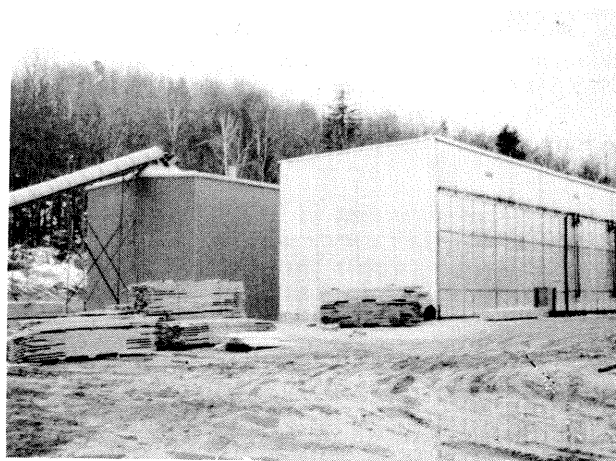
Figure 12.--A modern dry kiln at a New Hampshire sawmill uses an enclosed conveyor to carry wood residues to fuel the boiler system. (University of New Hampshire Department of Forest Resources).
