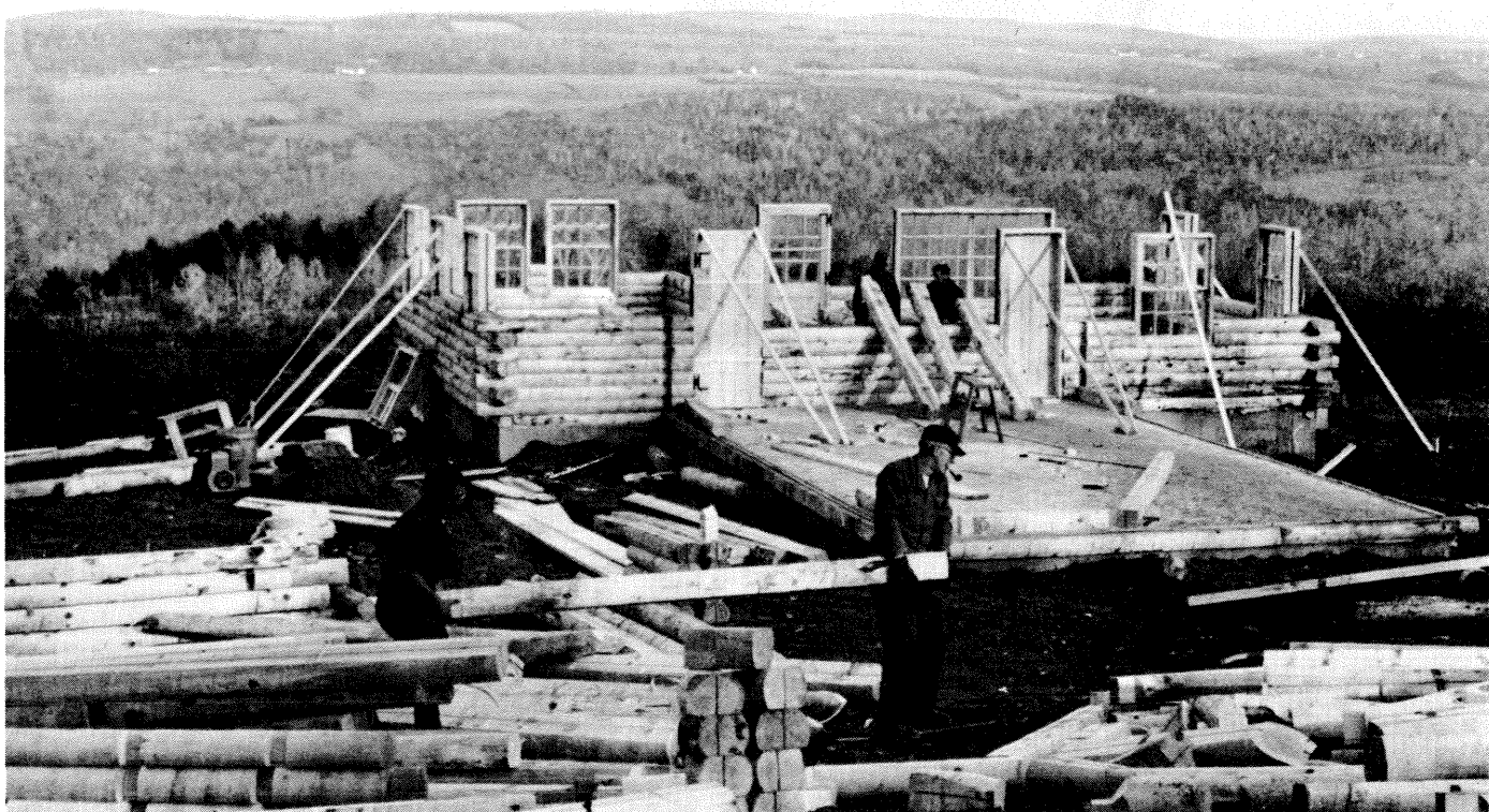
Figure 11.--Vermont's high-production log cabin manufacturers use most of the cabin logs produced in New Hampshire and Vermont. Here, one uses a four-man crew to erect a cabin on a prepared foundation in less than 4 days. (Vermont Department of Forests, Parks and Recreation).
