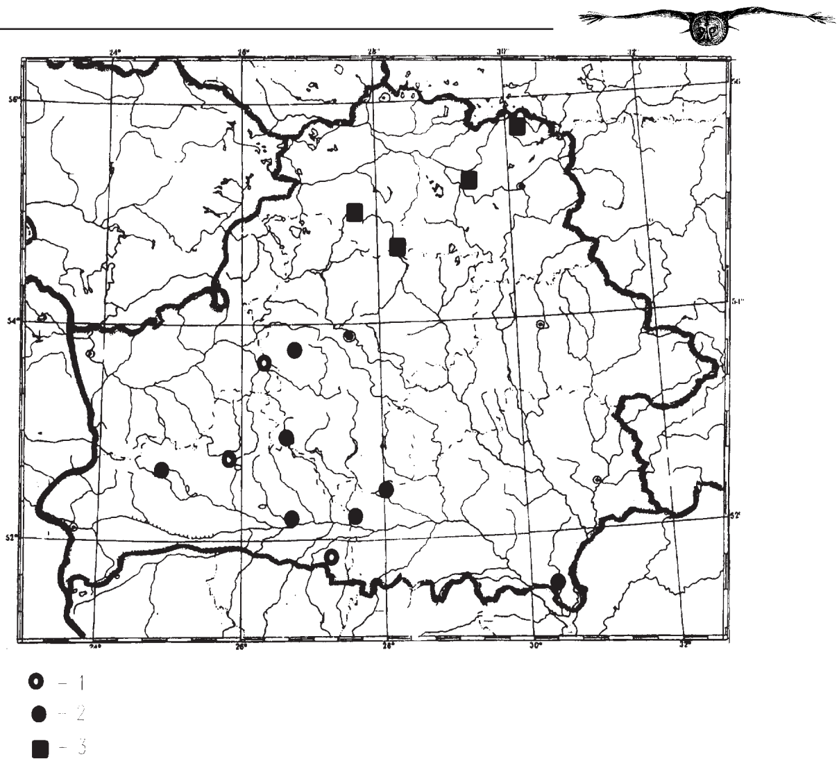
Figure 1. — Main sampling sites in dietary studies of Strix owls in Belarus, samples of no less than 75 prey items were collected in every site. 1 — Great Gray Owl ( Strix nebulosa ). 2 — Tawny Owl ( S. aluco ). 3 — Ural Owl ( S. uralensis ).
