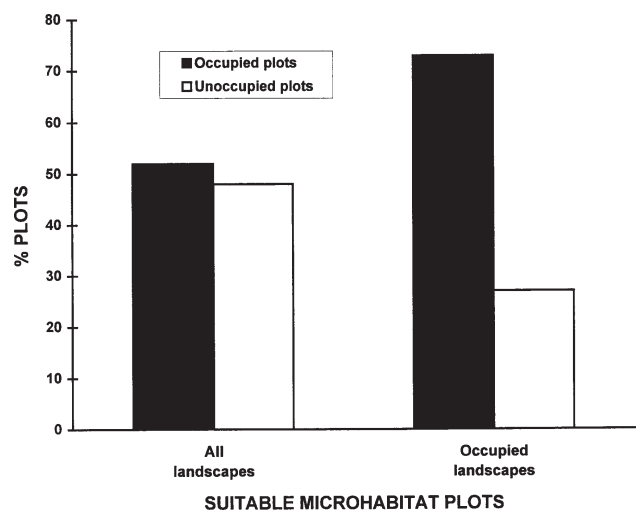
Figure 3.—Percent of suitable microhabitat (i.e., old-growth and mature ponderosa pine/Douglas-fir) plots occupied in all landscapes, compared to percent of suitable microhabitat plots occupied only in landscapes occupied by Flammulated Owls ( Otus flammeolus ), west-central Montana, USA.
