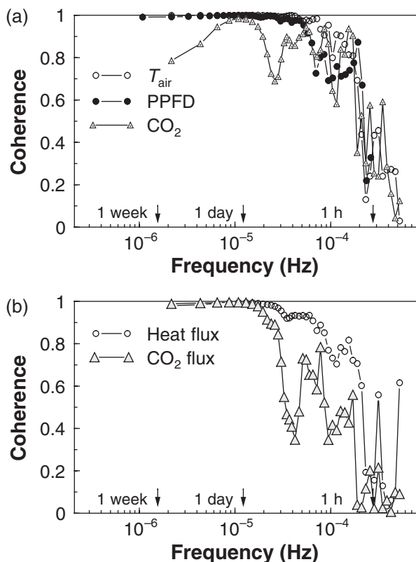
Fig. 2 (a) Coherence spectra for environmental variables recorded by systems on two towers separated by \sim 775 m show that fluctuations down to several hours are highly correlated. (b) Similar analysis for heat and carbon dioxide ( \text{CO}_2 ) fluxes indicate that even relatively high-frequency flux variations are correlated.
