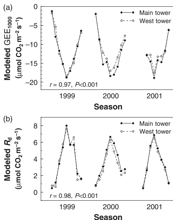
Fig. 4 Modeled GEE and nocturnal respiration obtained from simple models parameterized by independent data obtained from separate flux towers in similar forest.
