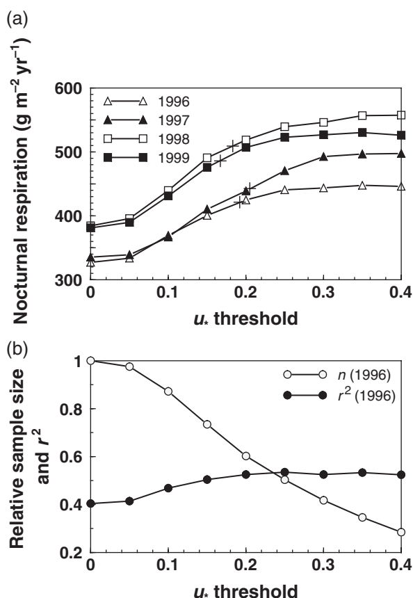
Fig. 14 (a) Annual estimates of nocturnal respiration as a function of u_{*} threshold for accepting data (only first 4 years shown for clarity). Estimates are relatively constant for u_{*} > 0.25 . The crosses indicate annual nocturnal respiration estimate using an alternative acceptance criteria of stability classe 4 or 5. (b) Relative sample size (open circles) and squared correlation coefficient of respiration model fit to nocturnal data (closed circles) as a function of u_{*} threshold.
