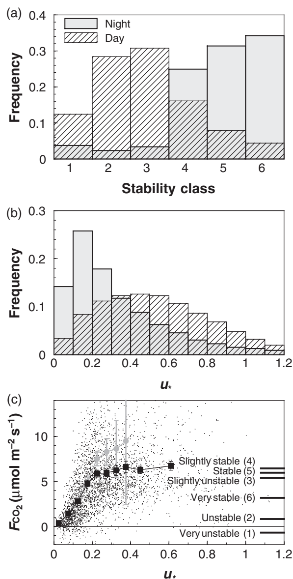
Fig. 13 (a) Frequency of occurrence of atmospheric stability classes, and (b) friction velocity ( u_* ) thresholds, by day and night at the Howland forest. The nocturnal atmosphere at Howland is characterized by stable conditions and low u_* values. (c) Nocturnal carbon dioxide (CO 2 ) flux for 15^\circ\text{C} < T_{\text{air}} < 18^\circ\text{C} . The square symbols ( \pm 95\% confidence intervals) represent 0.05 \text{ m s}^{-1} u_* classes, and the lines on the right side of the figure are the means of the six stability classes. The light gray circles ( \pm 95\% confidence intervals) indicate mean flux values if the u_* during the preceding half-hour was < 0.2 \text{ m s}^{-1} . Flux values are relatively constant with u_* > 0.25 and similar to values obtained for slightly or moderately stable conditions.
