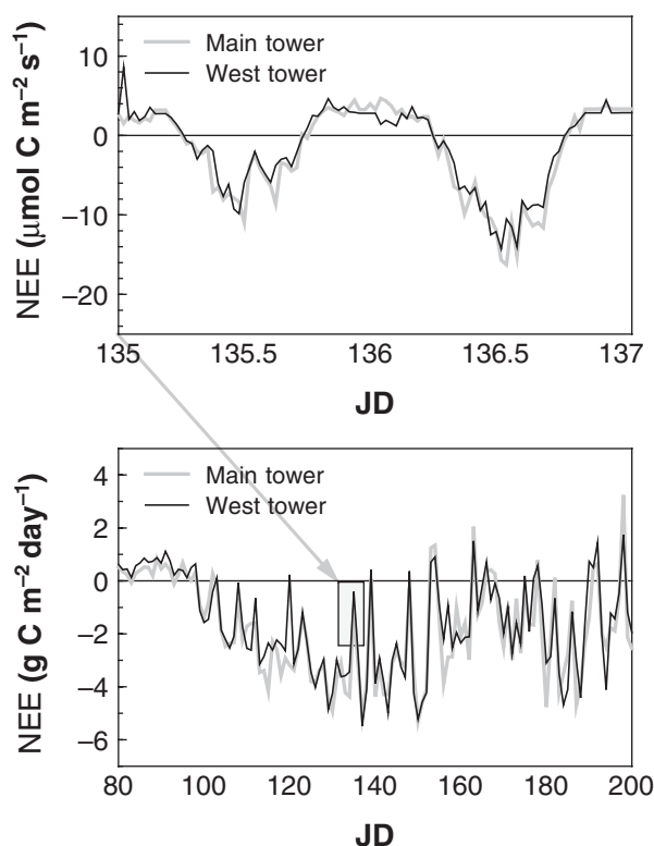
Fig. 1 Net ecosystem C exchange (NEE) fluxes recorded at two towers separated by \sim 775 m are correlated over short term as well as long term.
