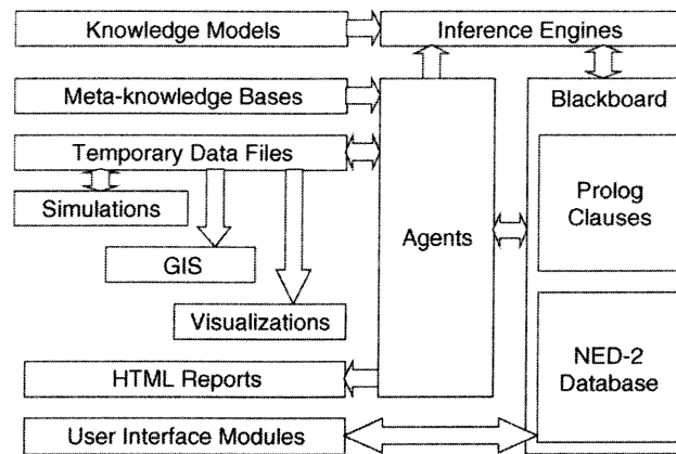
Fig. 1. The NED-2 architecture, a diagram illustrating the relationships among components of the agent-based design using a blackboard for communication between modules.
