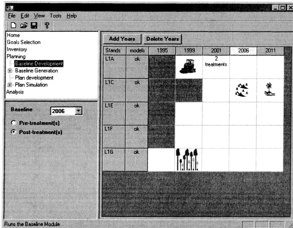
Fig. 4. A sample baseline development screen in NED-2 illustrates the graphical interface and hierarchical organization of selecting and simulating growth to a single, standardized baseline year.
