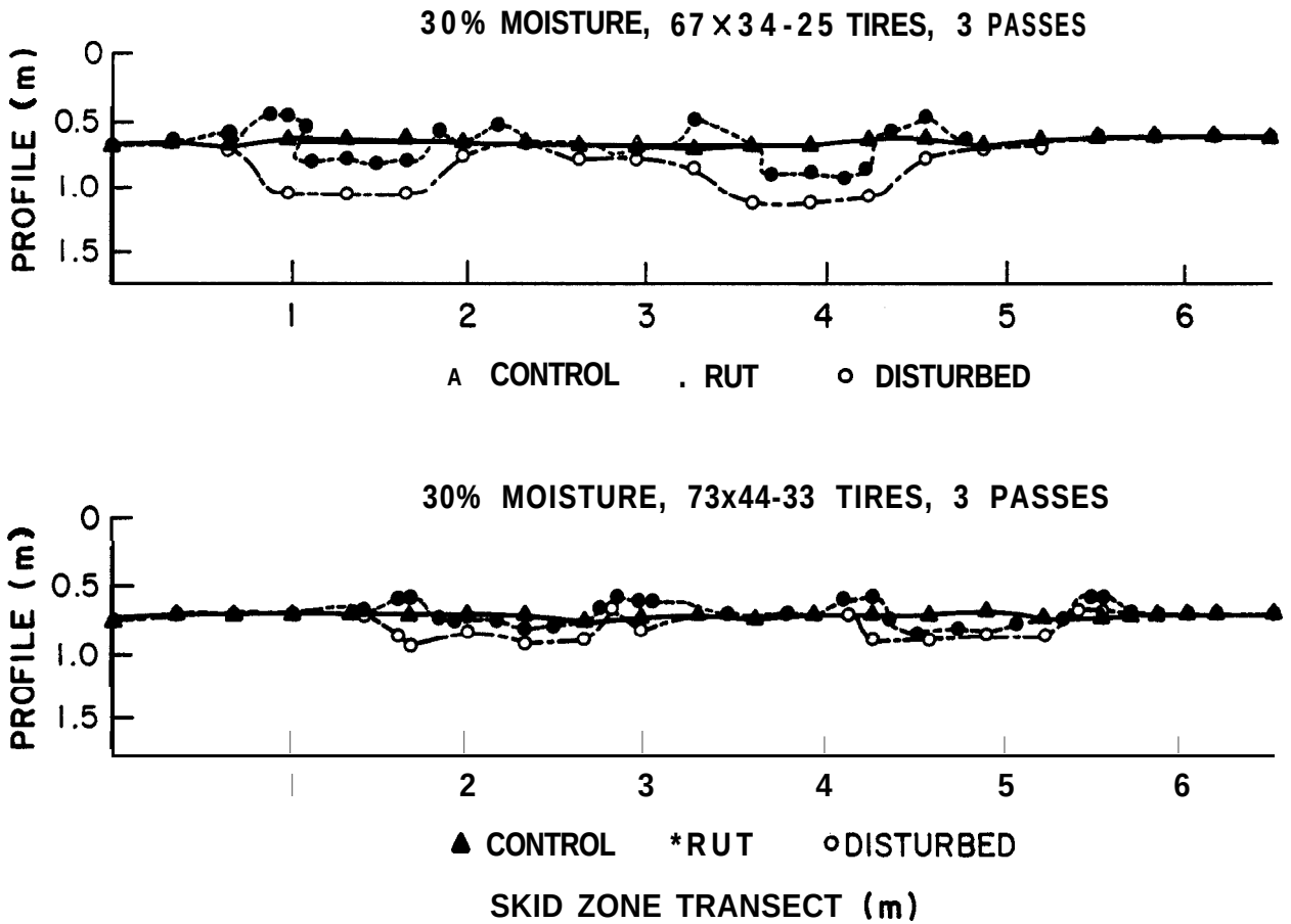
Figure 4.--Example of a skid zone profile comparing disturbance created by two different tire sizes.
