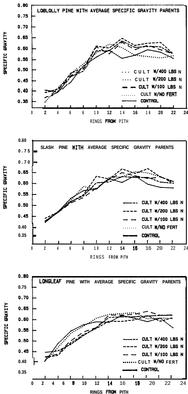
Figure 2.--Effect of intensive cultural treatment on ring specific gravity and length of juvenility for loblolly, slash, and longleaf pine average specific gravity progeny.
