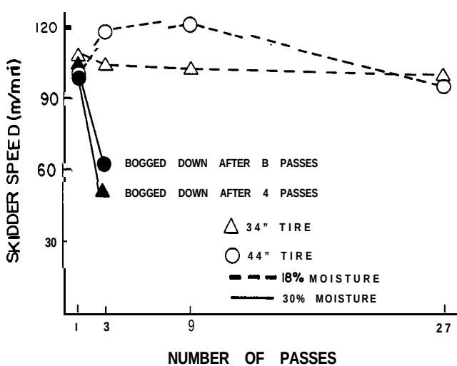
Figure 5.--Skidder speed as a function of soil moisture content, tire size, and number of passes.
