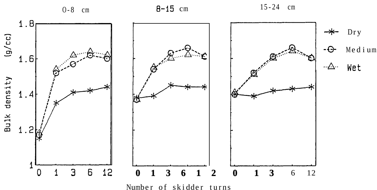
Figure 2. The changes in bulk density associated with number of skidder turns, soil moisture and depth
