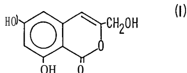
6,8-Dihydroxy-3-hydroxymethyl isocoumarin
