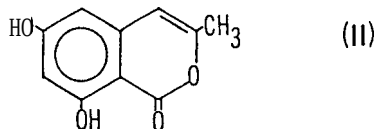
6,8-Dihydroxy-3-methyl isocoumarin
