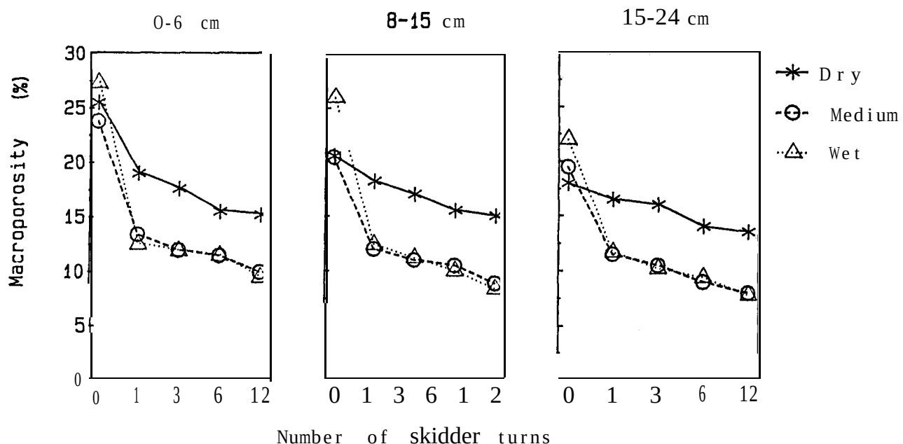
Figure 4. The changes in macroporosity associated with number of skidder turns, soil moisture and depth
