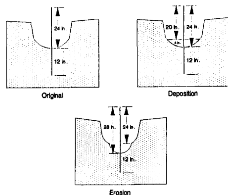
Figure 1. -- Cross section of a rut showing technique used for measuring soil movement
