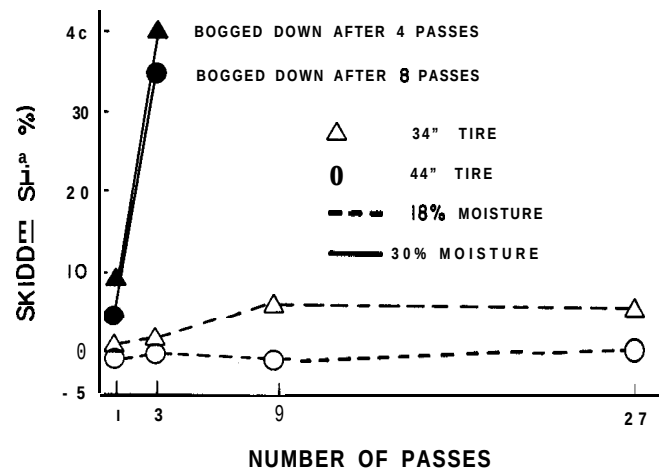
Figure 6.--Tire slip as a function of soil moisture content, tire size, and number of passes.
