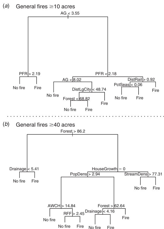
Fig. 7. Classification trees for (a) general fires \geq 4 ha (10 acres), and (b) general fires \geq 16 ha (40 acres). Variable abbreviations are defined in Table 1, and interpretation of the tree diagrams are described in Fig. 5.
