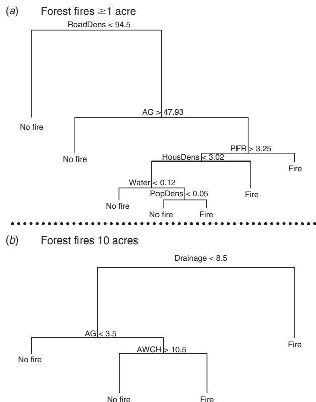
Fig. 6. Classification trees for (a) forest fires \geq 0.4 ha (1 acre), and (b) forest fires \geq 4 ha (10 acres). Variable abbreviations are defined in Table 1, and interpretation of the tree diagrams are described in Fig. 5.
