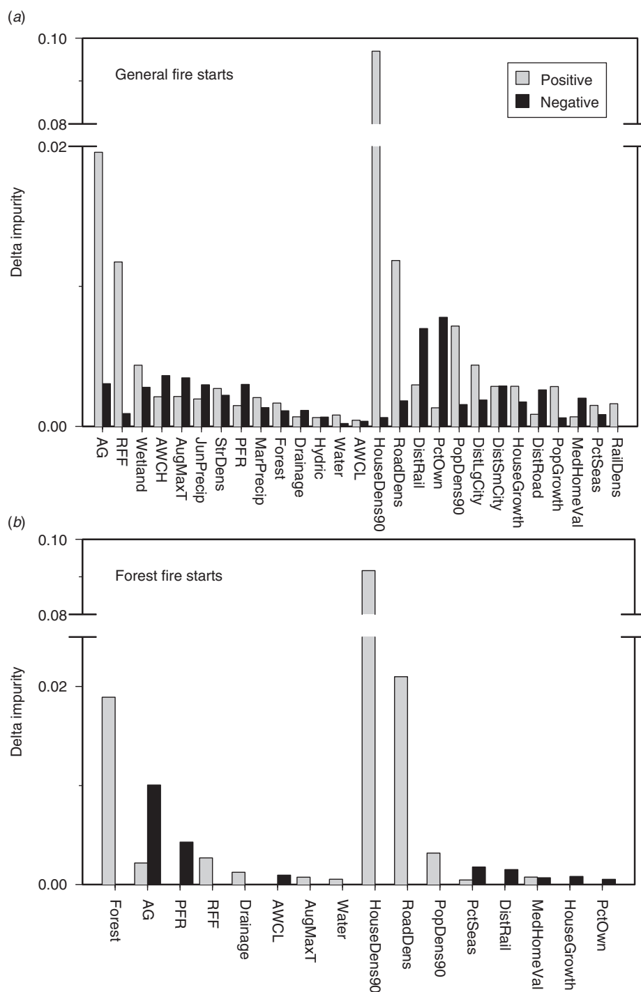
Fig. 4. Relative contribution of each independent variable, measured as the total decrease (delta) in impurity summed across all splits for both (a) general (i.e. all) fire observations, and (b) forest-specific fire observations. The direction of influence (i.e. positive or negative) of the variable indicates whether increasing the variable above the threshold value deciding the split increased or decreased the likelihood of observing a fire observation. Classification trees had (a) 306 for general fire observation and (b) 35 splits for fire observation models.
