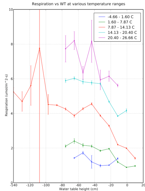
Figure 2: Lost Creek ER at different temperature ranges as a function of water table depth. The lessening of ER with deepening water table is most clear in the 7-14°C range, and appears to have a threshold at a water table depth of about 40 cm. below the soil surface. Error bars represent 95% confidence intervals.
