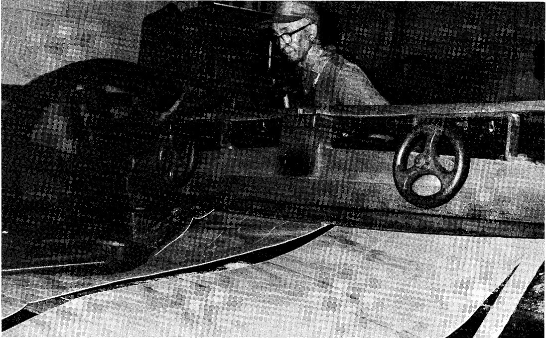
Figure 9. —Veneer is trimmed after being sliced. In 1965 West Virginia veneer manufacturers consumed nearly 6.4 million board feet of veneer logs.
