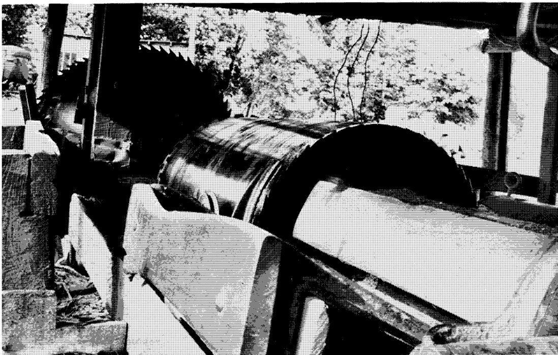
Figure 12.—A white oak stave leaves the saw. In 1965 West Virginia produced $575,380 worth of white oak cooperage bolts for the tight cooperage industry.
