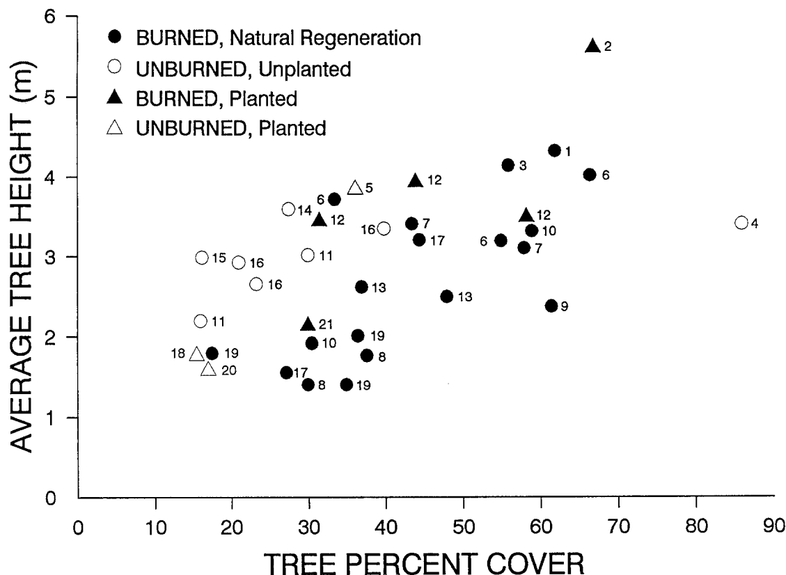
Fig. 2. Ranges of average tree height and percent tree canopy of stands sampled within habitat occupied by Kirtland's warblers in Michigan. Classification of habitats into marginal or suitable follows the categories defined for contrasting pairing success (Probst and Hayes, 1987). (Young marginal habitat matures into suitable.) 1. Artillery South; 2. Mack L. Red Pine #1; 3. Pere Cheney; 4. Ogemaw Management*; 5. Lovells N. (S.5); 6. Muskrat Lake (S.7, S.13N, S.13S); 7. Artillery North (S.8 and 9, S.9 South); 8. Damon* (North, South); 9. Fletcher Burn; 10. Mack L. Prescribed Burn (1978, 1983); 11. Mack L. Unburned (1980, 1983); 12. Mack L. Plantation (S.3) (Jack Pine, Red Pine); 13. Lovells South; 14. Monument; 15. McKinley #1; 16. McKinley (Area #2, Area #3, Area #4); 17. Rayburn; 18. Lovells North #2 (S.6); 19. Bald Hill (1982 S.20, 1983 S.20, 1983 S.14); 20. Mack Lake, Red Pine #2; 21. McKinley #5 ('77 Plantation). (*Data from Smith (1979).)
