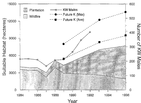
Fig. 7. Quantity of suitably-stocked habitat and proportion in plantation and wildfire for Kirtland's warbler in Michigan (1984–1996). Past populations (1984–1992) and estimated carrying capacity (1989–1996) of male Kirtland's warblers are also shown. The lower carrying capacity estimate is based on the 1984 average male density (1.9 males per 40 ha) in wildfire plus plantation habitat. The higher estimate (2.8 males per 40 ha) was derived from peak populations during the middle years of habitat occupancy (see Fig. 1). Sources: Habitat area from unpublished reports by J. Weinrich (Michigan DNR) and D. Sorenson (USDA Forest Service).
