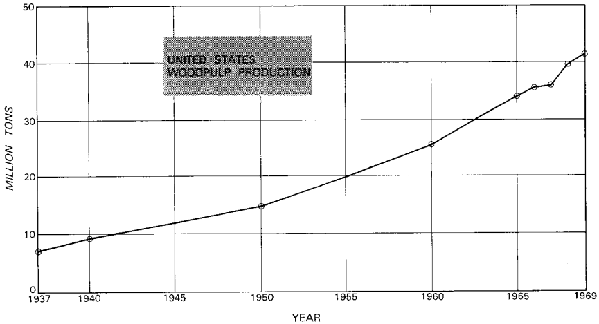
Figure 2.—U. S. woodpulp production for selected years 1937-1969.
