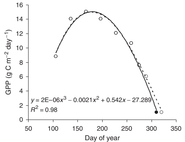
Fig. 5 The daily gross primary production for a closed canopy P. x euramericana growing at 550 ppm [CO 2 ] from the modeled data of Wittig et al. (2005). The cubic relationship between daily GPP and day of year in elevated [CO 2 ] is displayed (---). Advancing the end date by 10 days is represented (—) and the influence of this on seasonal GPP is calculated as the difference between the areas under the two curves. The result is an estimate of the seasonal GPP contributed from lengthening of the autumnal phenophase as a consequence of increased atmospheric [CO 2 ].
